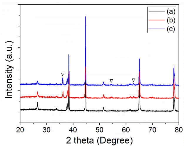
Fig. S1 XRD patterns of (a) FTO glass, (b) rutile NR array on FTO glass, (c) HNT array on FTO glass. ( \nabla the rutile peaks)
