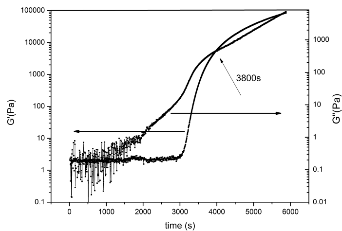
Figure S1 Rheological behavior of BTI123 at 120 °C
