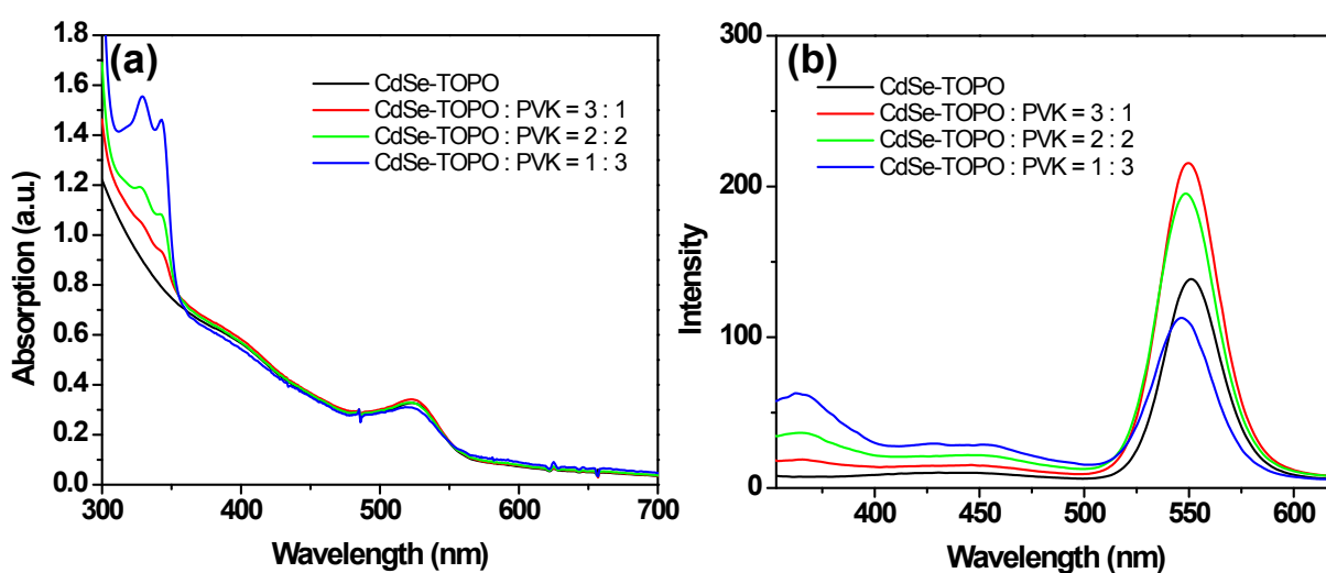
Fig. S1. (a) UV-Vis absorbance and (b) PL spectra of CdSe-TOPO, CdSe-TOPO and PVK mixtures in THF (3:1, 2:2, 1:3 in weight). Total concentration of each solution is 1 mg/ml.
