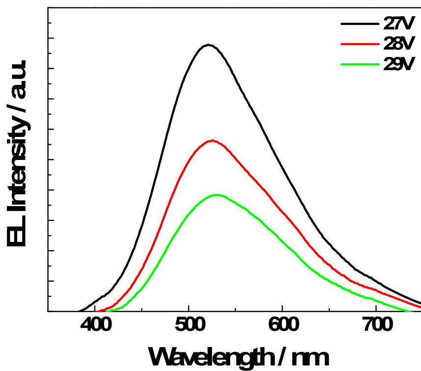
Fig. S2. EL spectra of QD-LED with configuration of ITO/PEDOT:PSS/PVK:PBD:QD(1wt%)/LiF/Al with increasing applied bias voltages (27V - 29V).
