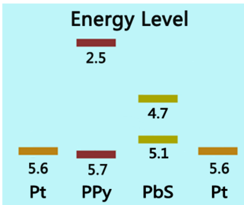
Figure S1. Energy level diagram of PbS and PPy (eV).
