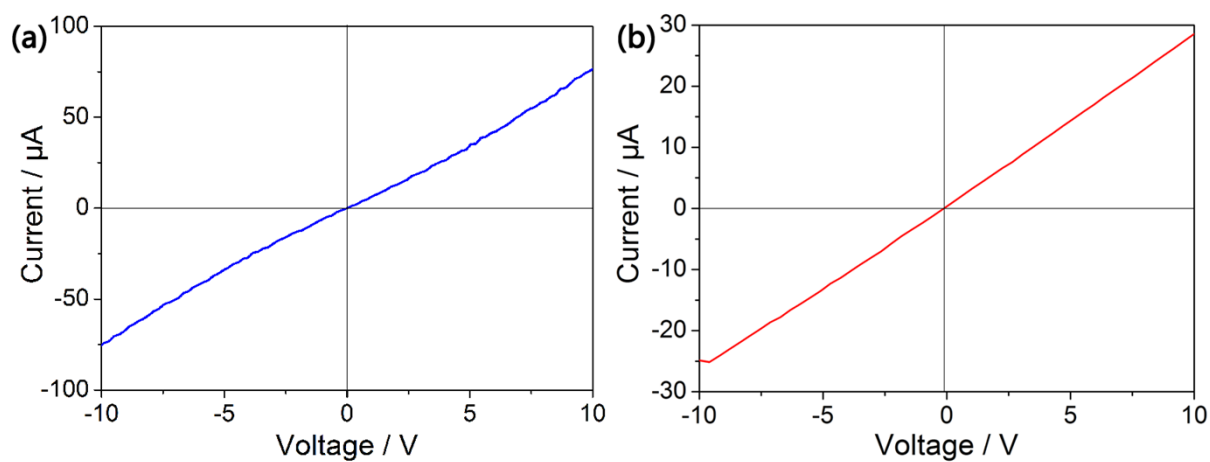
Figure S2. I-V curves of PbS (a) and PPy (b) nanowire devices.
