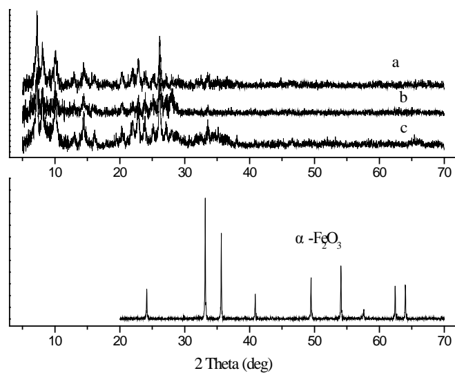
XRD patterns of Fe 2 O 3 /HMCM-49 with various supporting loadings a: 0.32%; b: 0.69%; c: 5.04%
