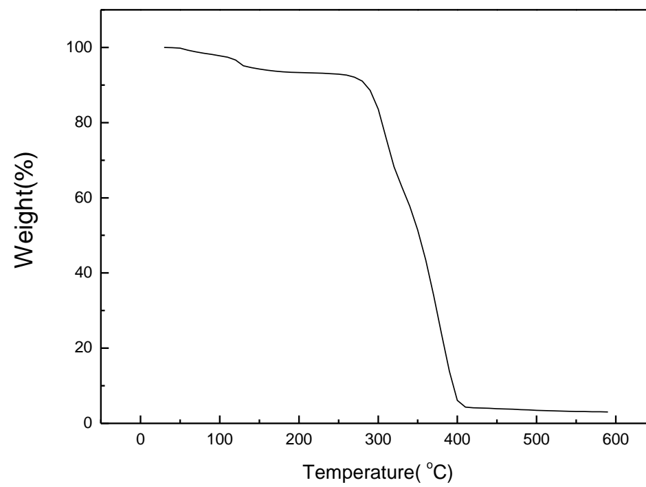
Figure S5. TG curves for [DDPA][Tos]
