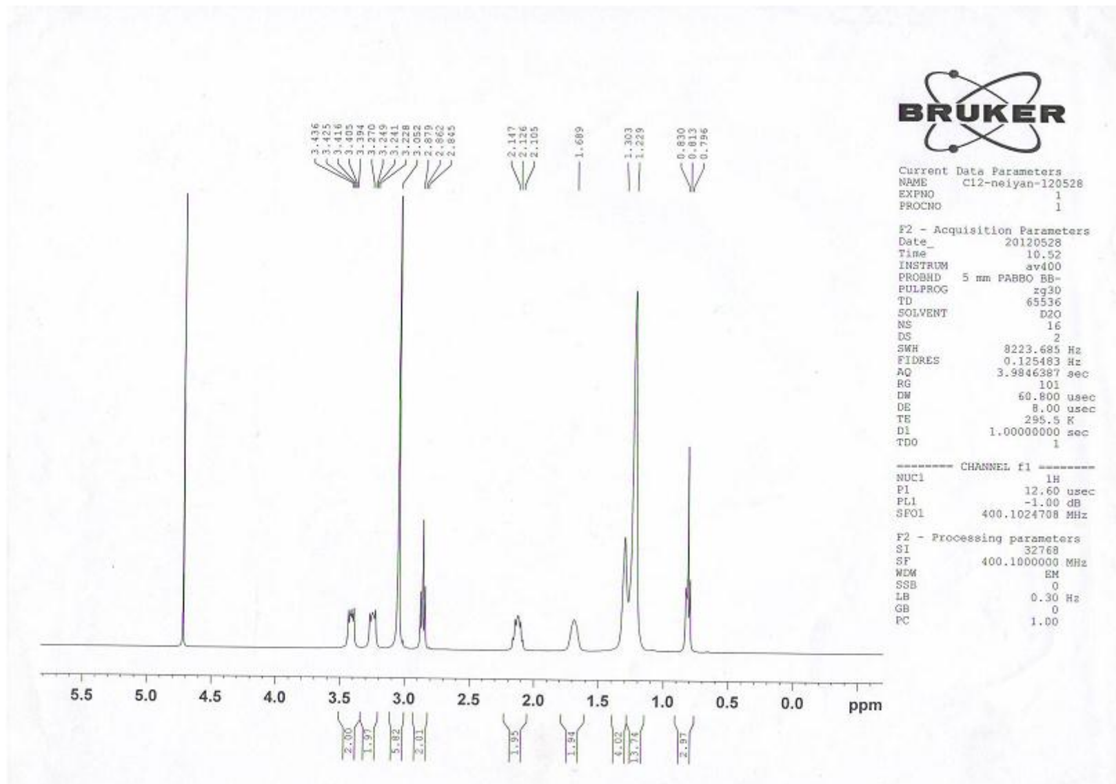
Figure S2. 1 H NMR Spectrum of DDPA
