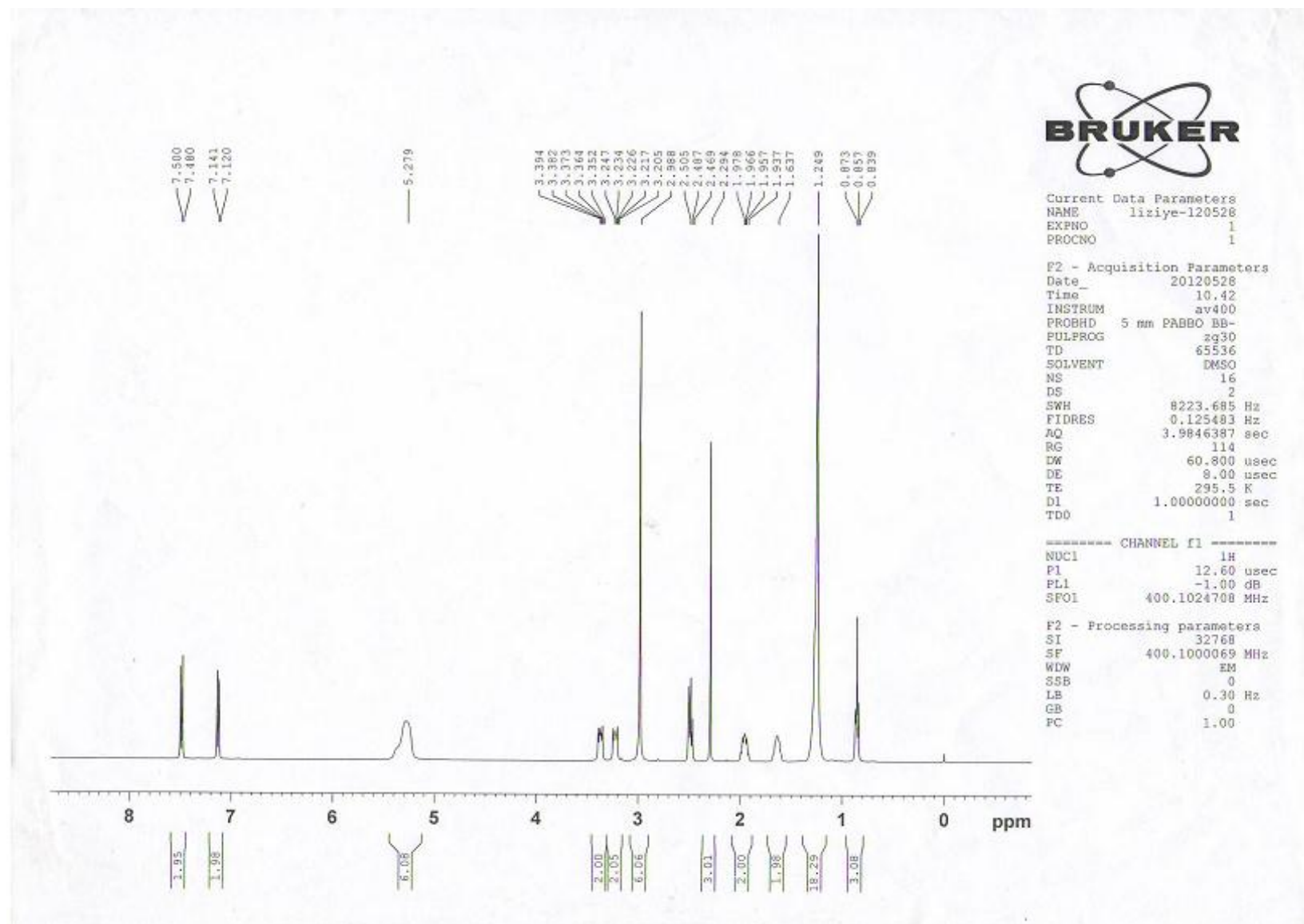
Figure S1. ^1\text{H} NMR Spectrum of [DDPA][Tos]
