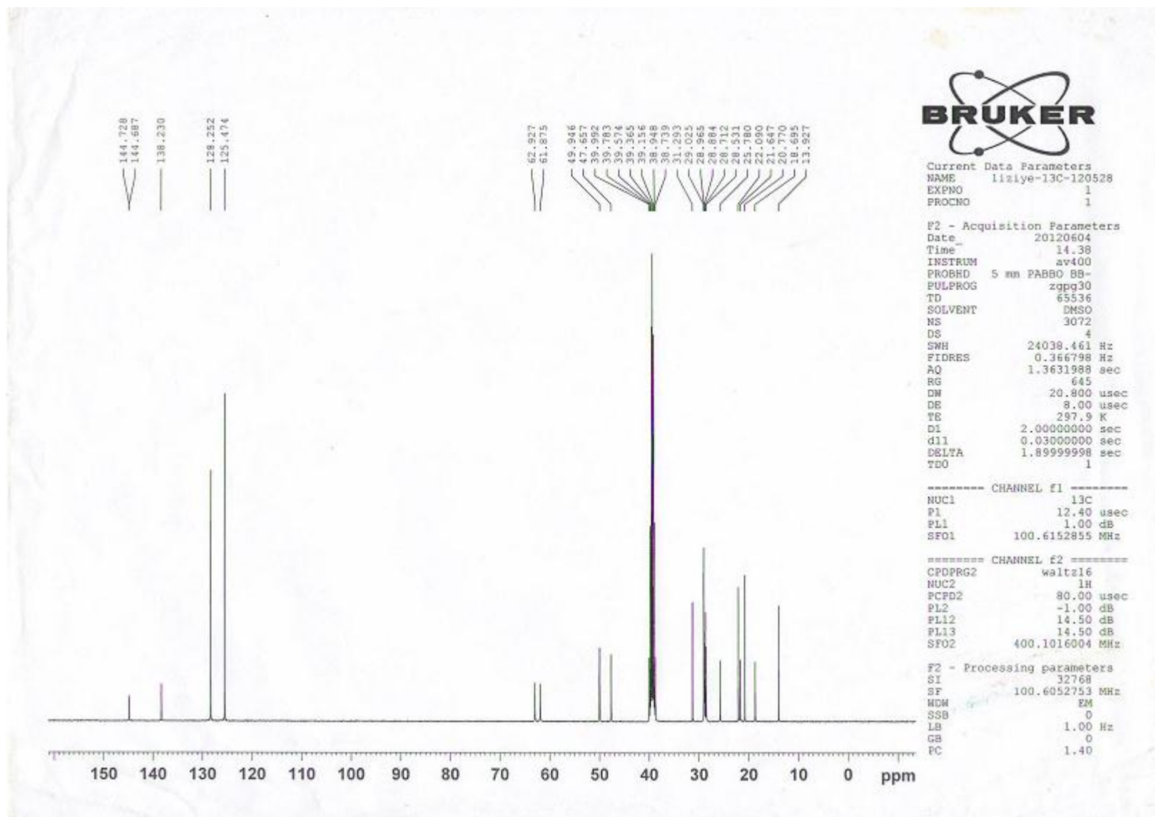
Figure S3. ^{13}\text{C} NMR Spectrum of [DDPA][Tos]
