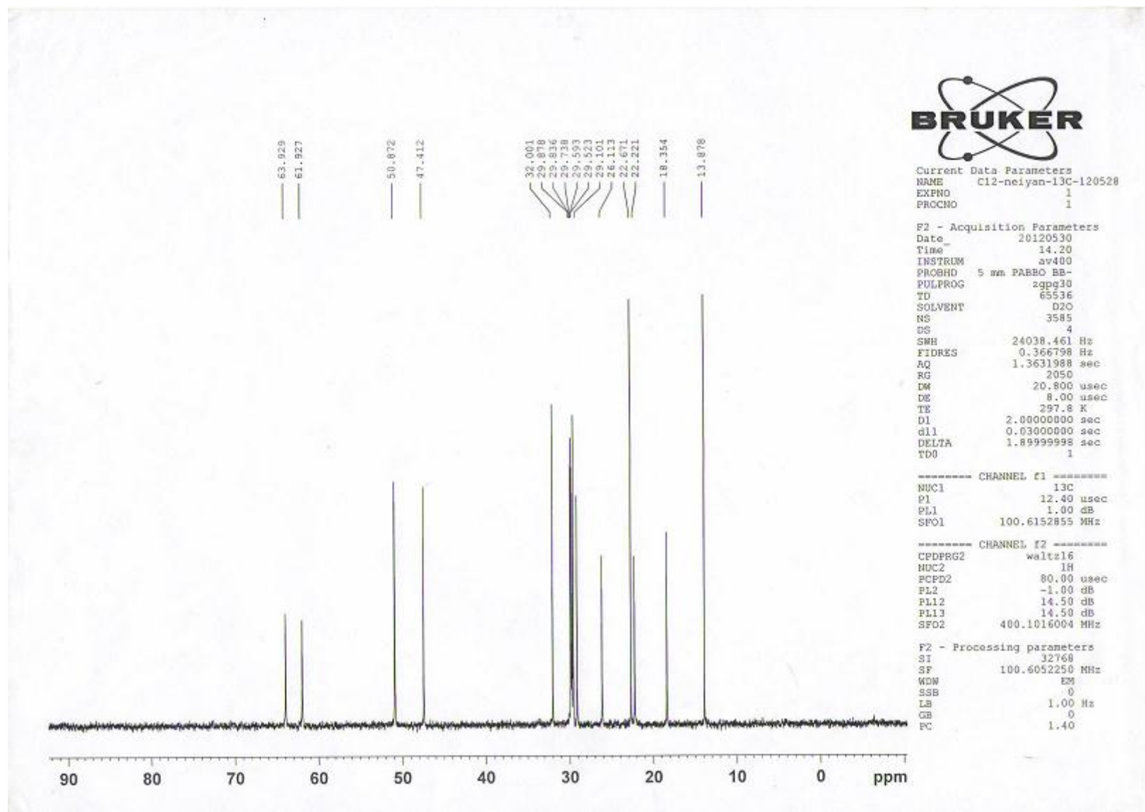
Figure S4. ^{13}\text{C} NMR Spectrum of DDPA
