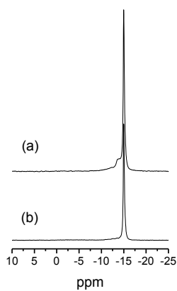
Figure S3 1 H-decoupling 31 P MAS NMR spectra of (a) Al 0.1 CsPW and (b) CsPW after the adsorption of 2- 13 C-acetone.
