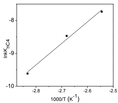
Figure S2 Arrhenius plot for 1- 13 C-n-butane isomerization over Al 0.1 CsPW.
