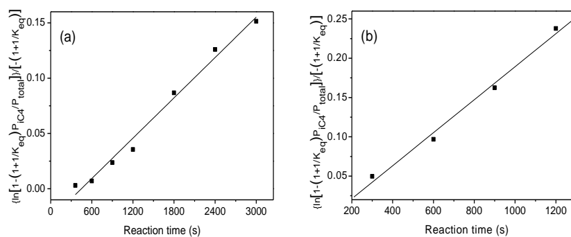
Figure S1 The plots of rate constants for 1- 13 C-n-butane isomerization reaction obtained from eq. (2) over CsPW (a) and Al 0.1 CsPW (b).
