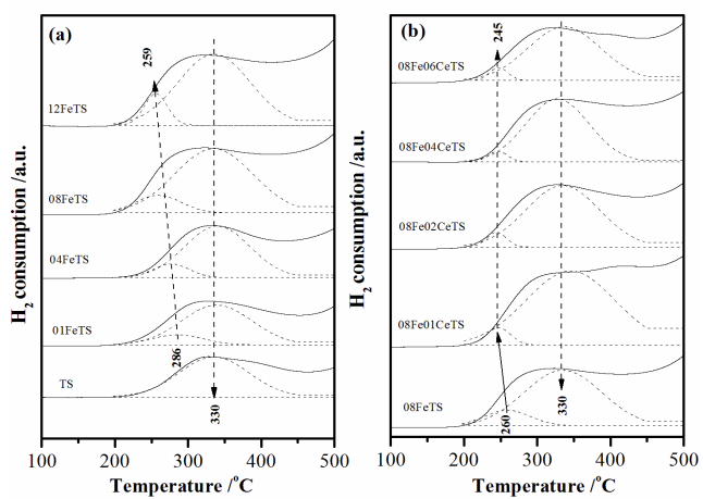
5 Figure S2 \text{H}_2 -TPR profiles of (a) x\text{FeTS} (b) 08\text{Fe}_y\text{CeTS} catalysts ( x = 0, 01, 04, 08, 12 ; y = 0, 01, 02, 04, 06 )
