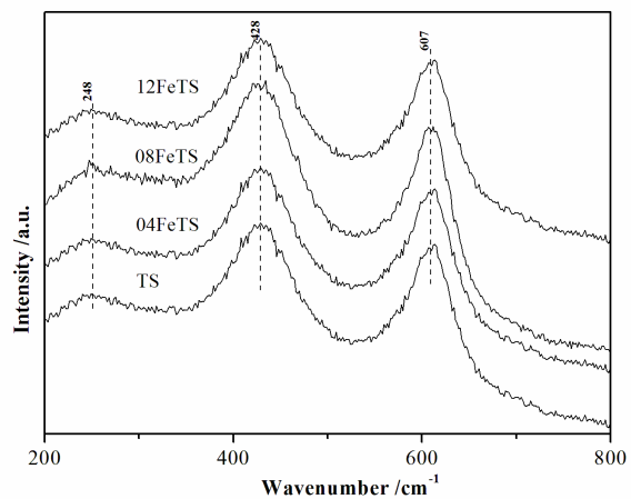
Figure S1. Raman spectra of x\text{FeTS} samples ( x = 0, 04, 08, 12 )
