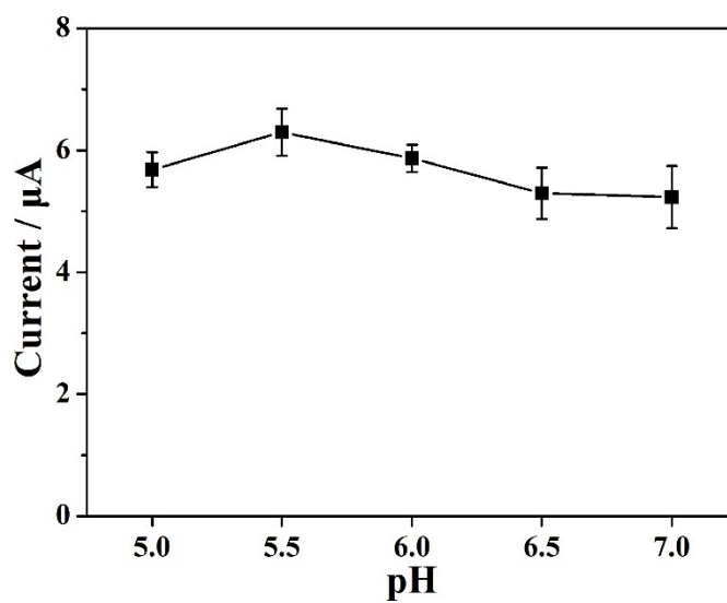
Fig. S9 Effect of the pH of HAc-NaAc buffer solution on the response current of the MCS@UiO-66-NH 2 /Lac/ABTS/CHIT/GCE biosensor.
