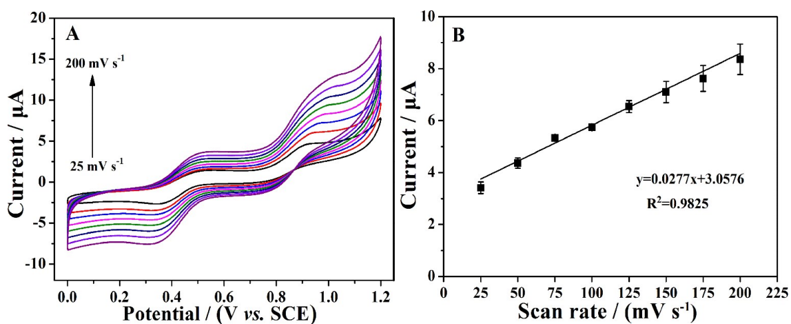
Fig. S6 (A) CVs of MCS@ UiO-66-NH 2 /Lac/ABTS/CHIT/GCE biosensor measured at scan rates range 25-200 \text{mV s}^{-1} . (B) Plots of the peak current vs. scan rate
