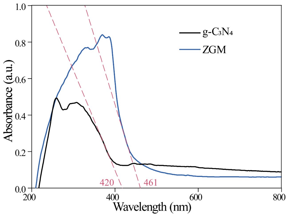
Fig. S2. UV-Vis diffuse reflectance spectra of ZGM and g-C 3 N 4 .
