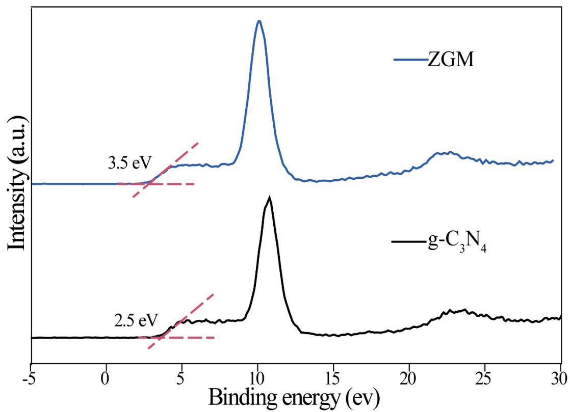
Fig. S4. Valance band XPS spectra of ZGM and g-C 3 N 4 .
