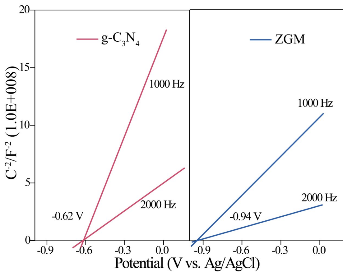
Fig. S3. Mott-Schottky plots of ZGM and g-C_3N_4 .
