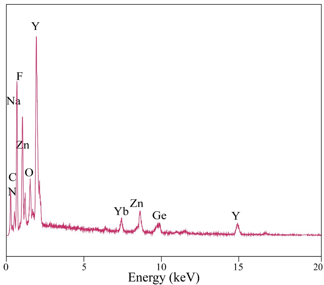
Fig. S1. The EDS spectrum of UZC.
