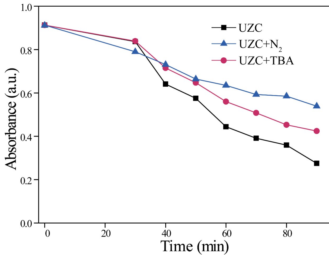
Fig. S5. The degradation curves of RhB with different treatments.
