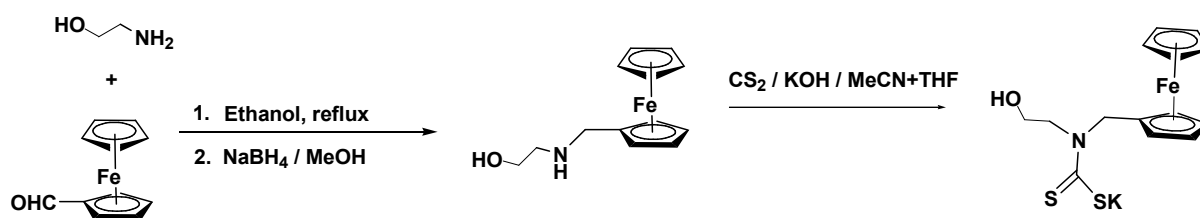
Scheme S1. Synthetic routes for the ferrocenyl dithiocarbamate ligand.
