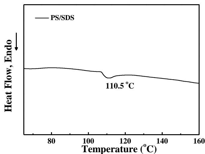
FIG S1. DSC heating curves of PS containing 1 wt% SDS without CNT sponges.
