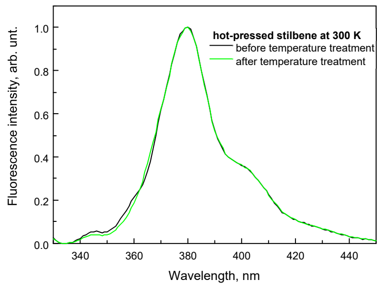
Figure S2. Normalized fluorescence ( \lambda_{\text{ex}}=300 nm) spectra of hot-pressed stilbene before temperature treatment (black line) and after low temperature treatment (green line) at 300K.
