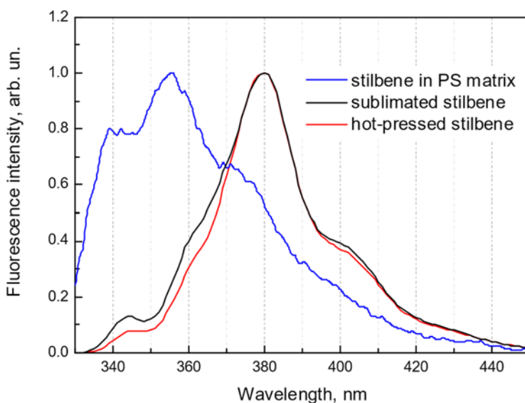
Figure S1. Normalized fluorescence ( \lambda_{\text{ex}}=300 nm) spectra of stilbene in PS matrix (blue line), of sublimated stilbene (black line) and of hot-pressed stilbene (red line) at 300K.
