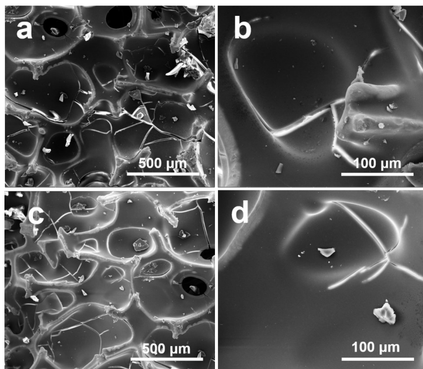
Fig. S1 SEM images of Carbide-filled NF before (a, b) and after (c, d) the hydrothermal experiment.
