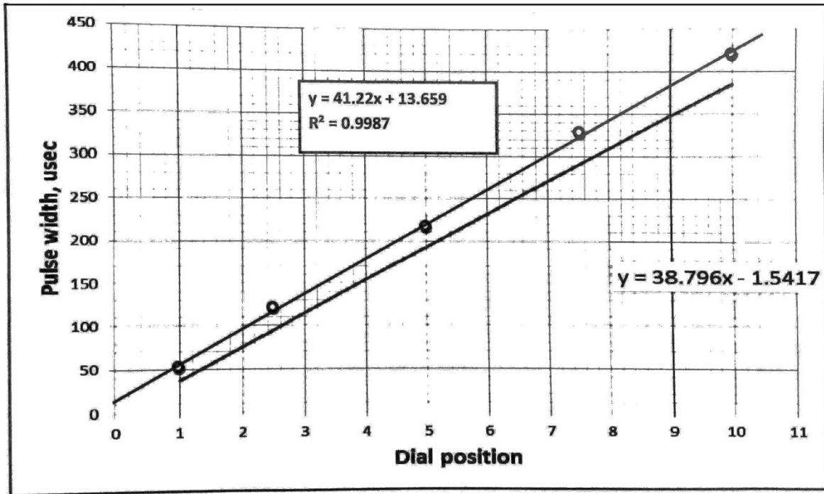
Fig. 2 Pulse width used in the FLS 980 Edinburgh instrument.
