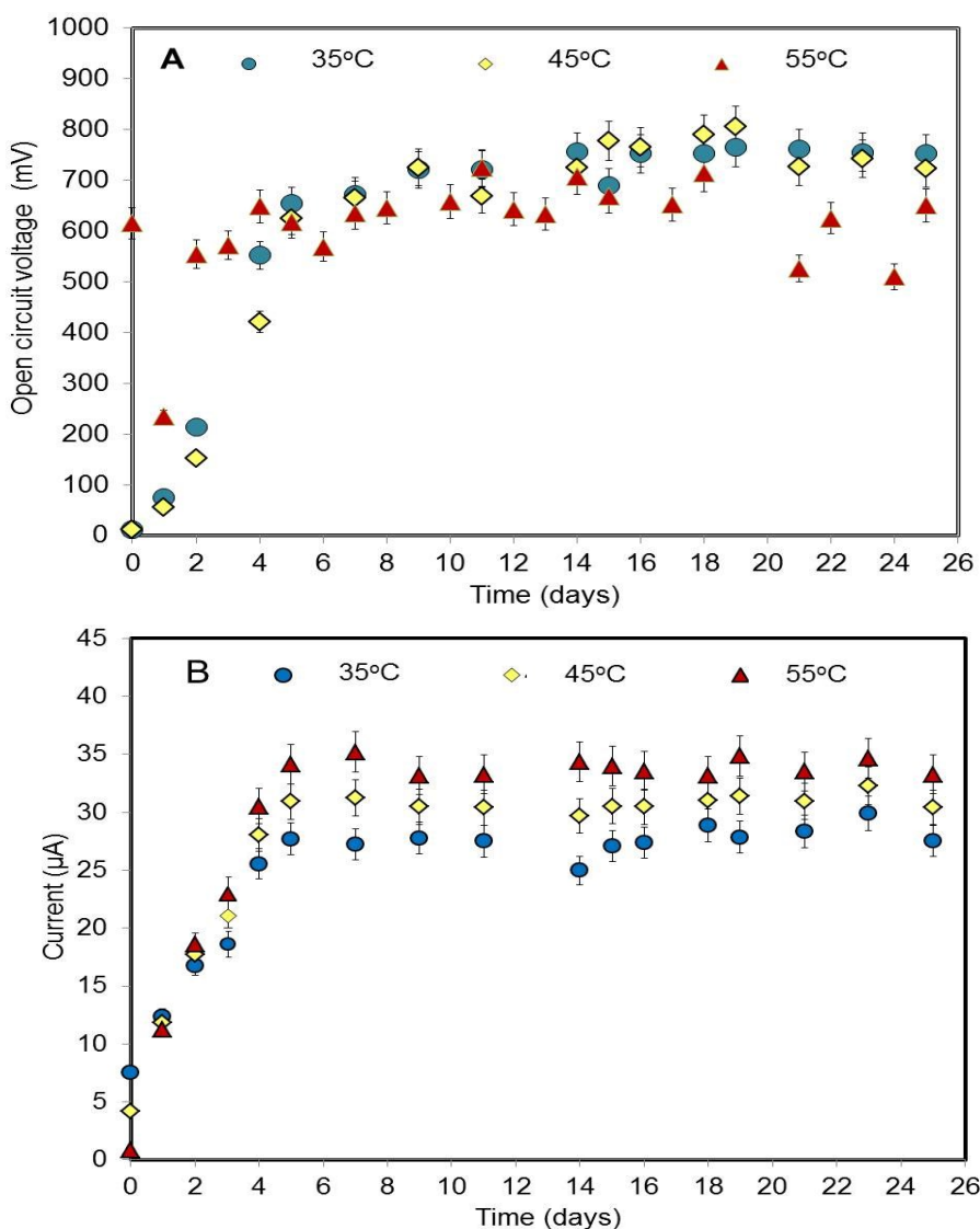
Fig. S1. Open circuit voltage (OCV) (A) and current (B) of MFCs for inoculated stage at different temperatures of 35, 45, and 55°C at start-up stage (CEM membrane as separator, carbon graphite mesh anode, and carbon graphite plate cathode).
