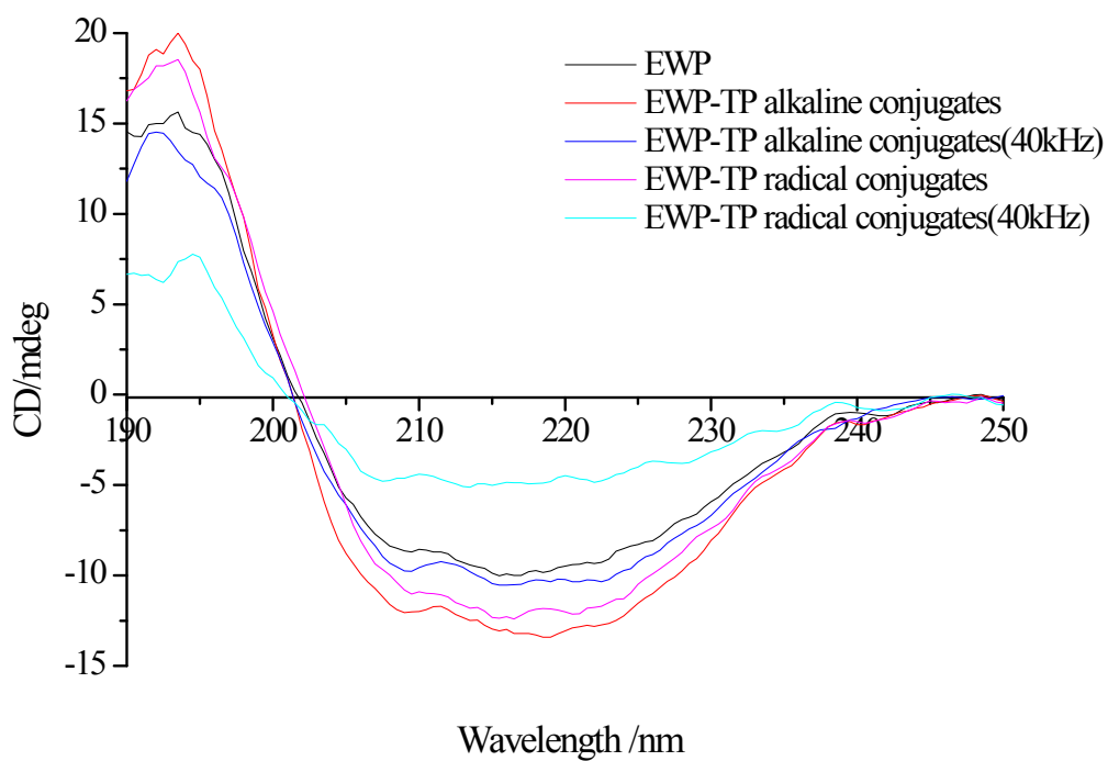
Figure 1 CD spectra of EWP and EWP-TP conjugates
