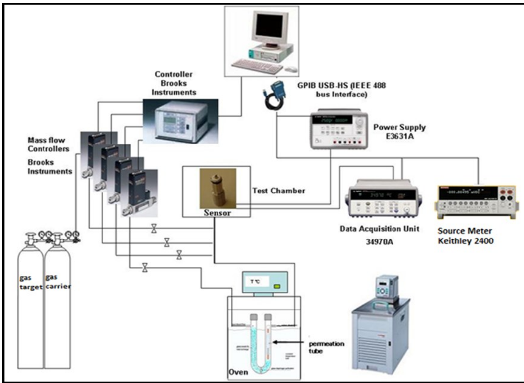
Fig. 1 Schematic diagram of the gas sensing setup used.
