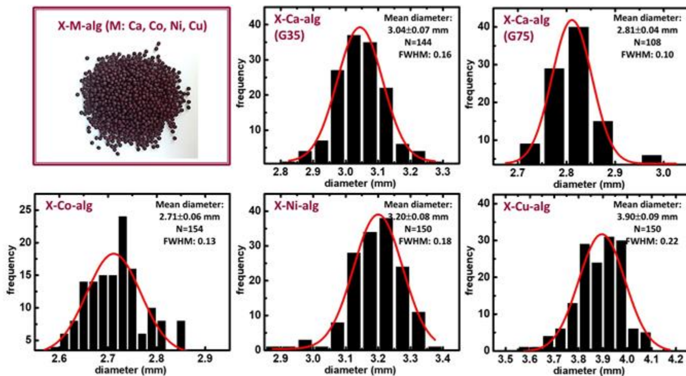
Figure S2. Optical photograph and size distributions of crosslinked X-M-alginate (M: Ca, Co, Ni, Cu), as indicated (diameters measured with ImageJ; histograms were calculated using OriginPro 9.0). Mean diameter and sample size (N) are shown on the Figure.
