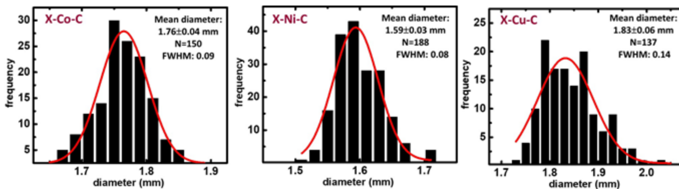
Figure S6. Size distributions of carbon (X-M-C) aerogel beads (M: Co, Ni, Cu), as indicated (diameters measured with ImageJ; histograms were calculated using OriginPro 9.0). Mean diameter and sample size (N) are shown on the Figure.
