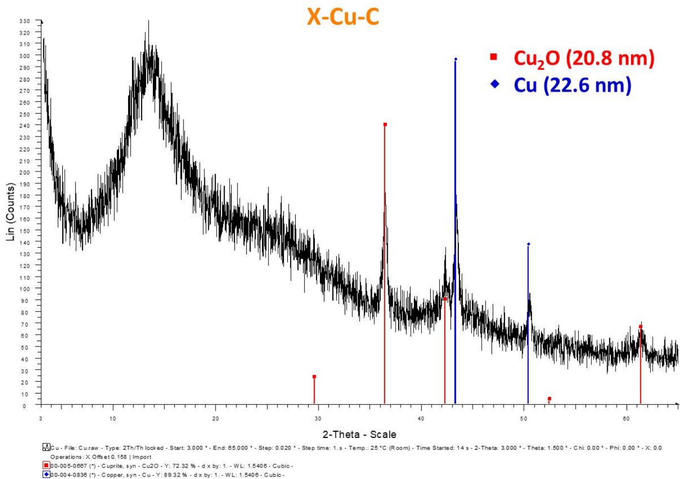
Figure S9. PXRD patterns of X-Cu-C aerogel beads. Simulated experimental spectrum and library line spectra. The crystallite size is shown in parentheses.
