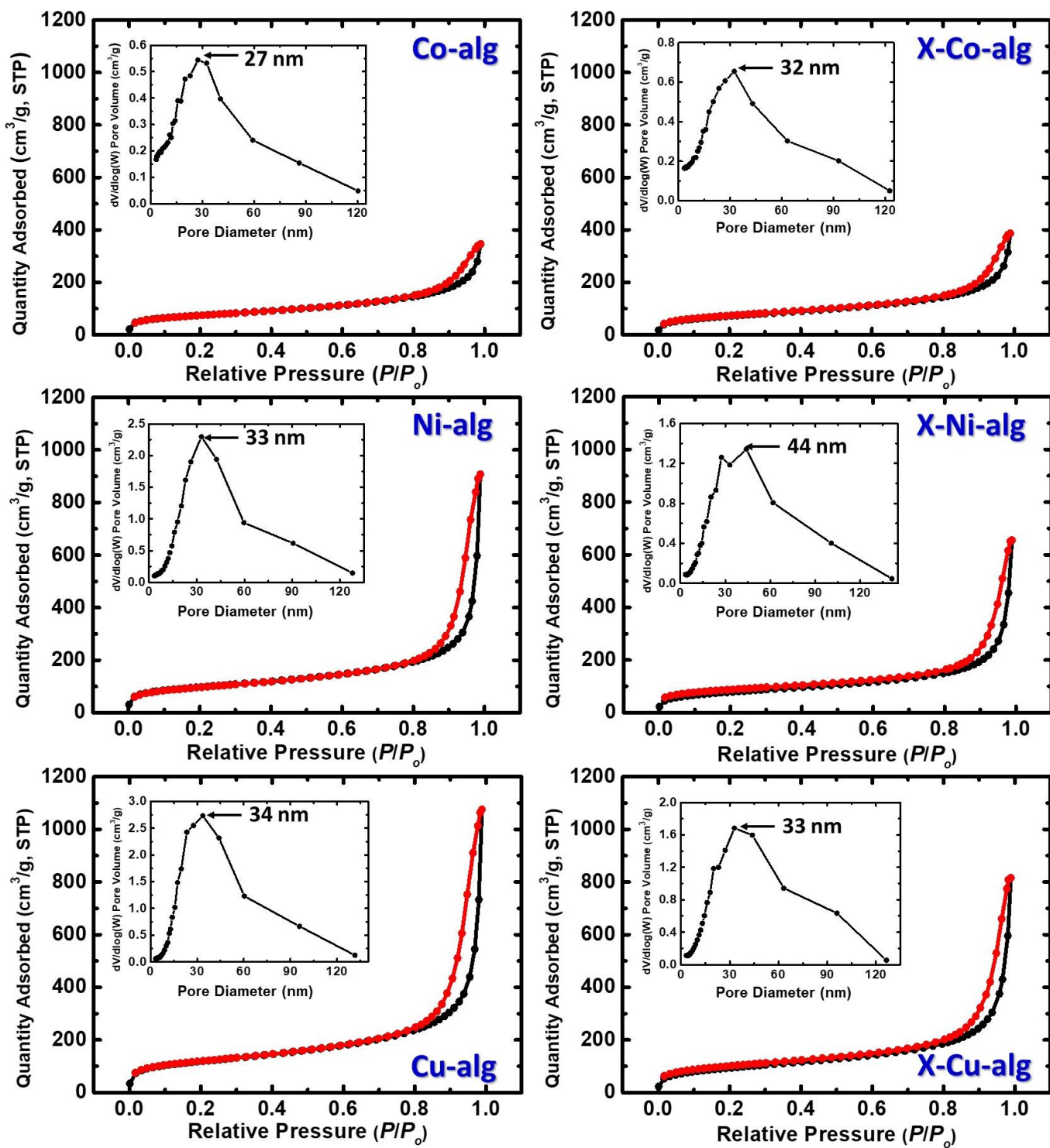
Figure S4. N 2 -sorption diagrams of native (M-alg – left) and crosslinked (X-M-alg – right) aerogel beads (M: Co, Ni, Cu), as indicated. Insets show pore size distributions by the BJH method.
