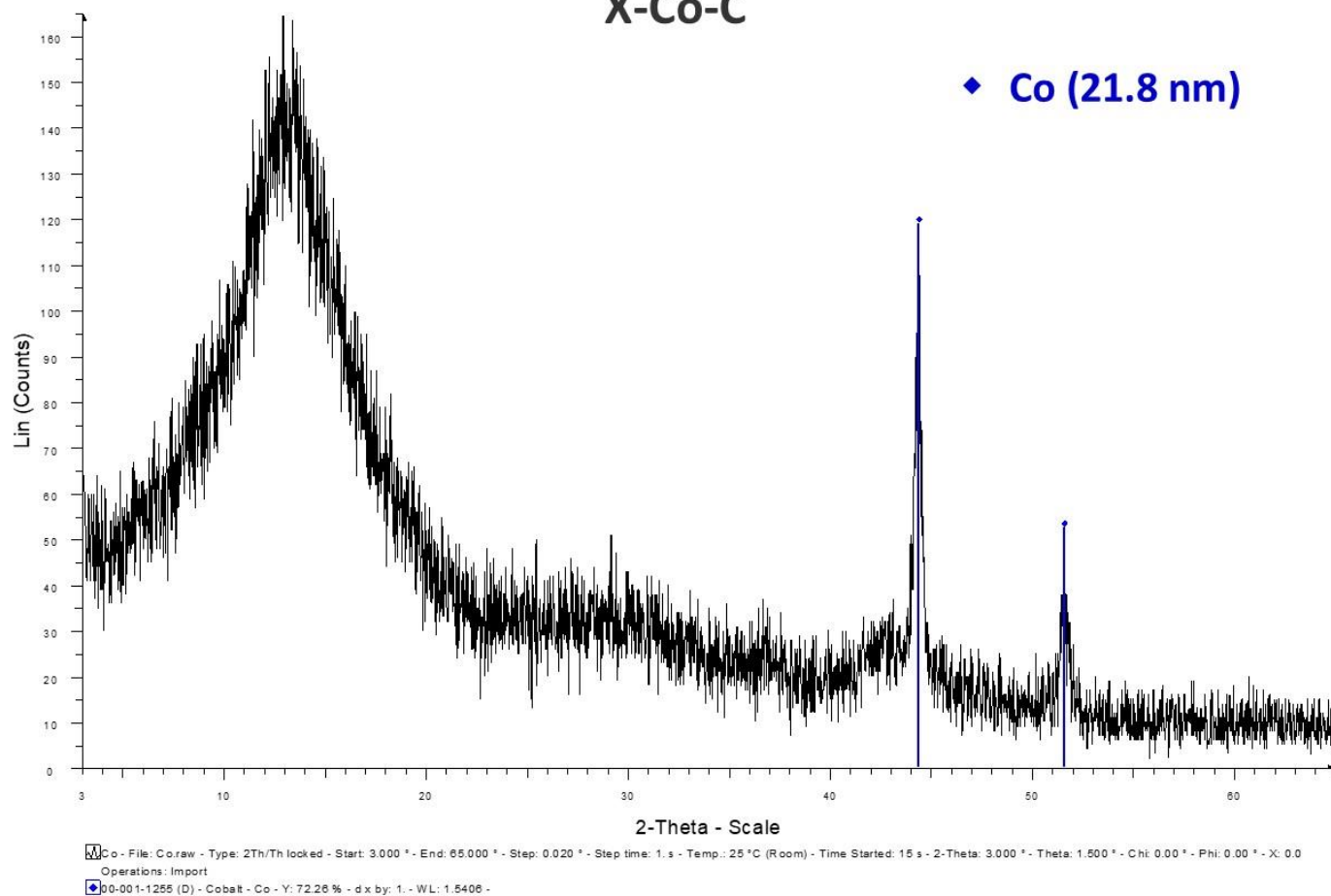
Figure S7. PXRD patterns of X-Co-C aerogel beads. Simulated experimental spectrum and library line spectra. The crystallite size is shown in parentheses.
