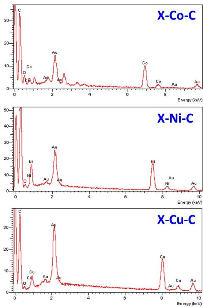
Figure S13. EDX spectra of carbon (X-M-C; M: Co, Ni, Cu) aerogel beads, as indicated.
