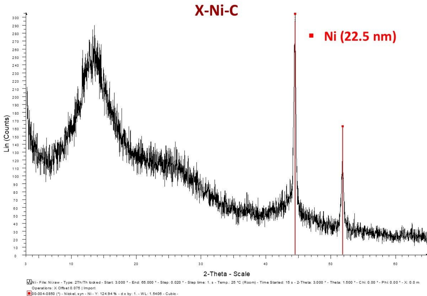
Figure S8. PXRD patterns of X-Ni-C aerogel beads. Simulated experimental spectrum and library line spectra. The crystallite size is shown in parentheses.
