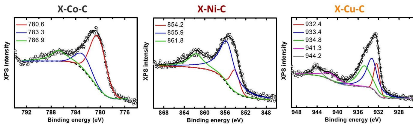
Figure S12. Deconvoluted Co 2p_{3/2} (left), Ni 2p_{3/2} (middle) and Cu 2p_{3/2} (right) XP spectra of carbon (X-M-C; M: Co, Ni, Cu) aerogel beads, as indicated. Experimental points are shown with black circles, cumulative fit plots with black solid lines and Shirley baseline with dashed black lines. Peak maxima (eV) are provided within the frames.
