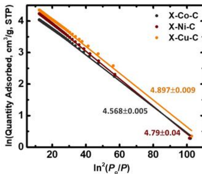
Figure S15. Dubinin-Radushkevich (DR) plots for carbon (X-M-C; M: Co, Ni, Cu) aerogel beads, as indicated. Specific micropore volumes were calculated from the intercepts (shown on the Figure, next to the corresponding line) of the linear-fitting plots.
