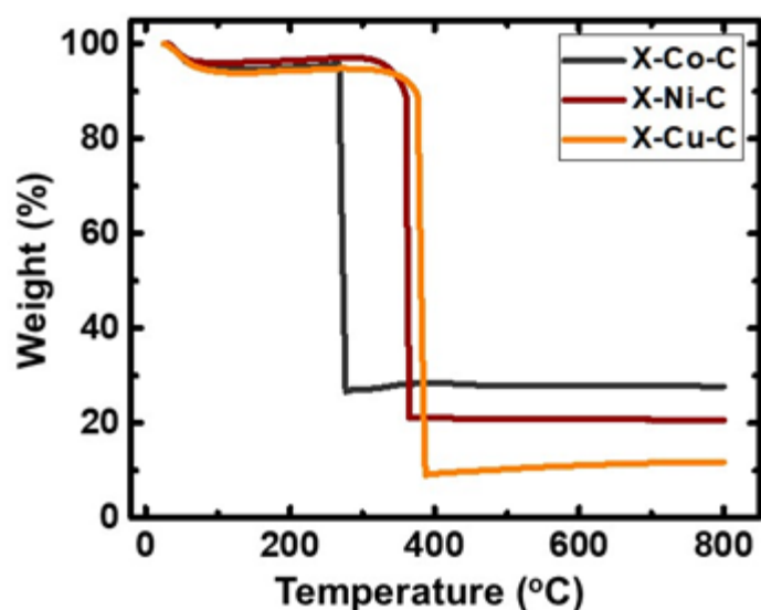
Figure S10. Thermogravimetric analysis (TGA, under O 2 ) of carbon (X-M-C; M: Co, Ni, Cu) aerogel beads, as indicated.
