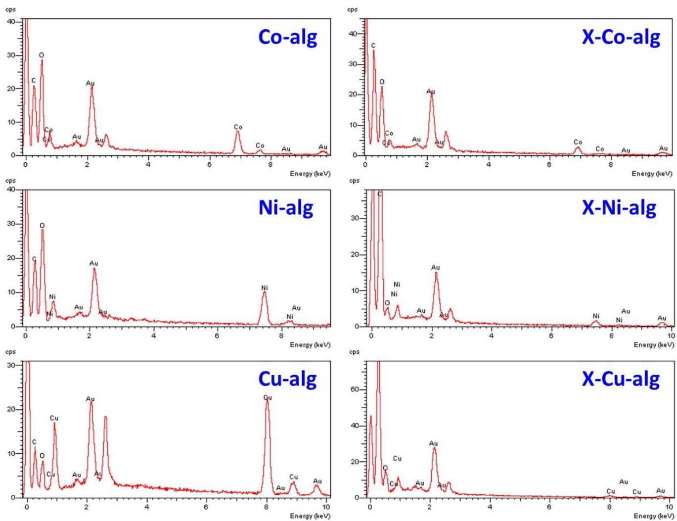
Figure S3. EDX spectra of native (M-alg) and crosslinked (X-M-alg) aerogel beads (M: Co, Ni, Cu), as indicated.
