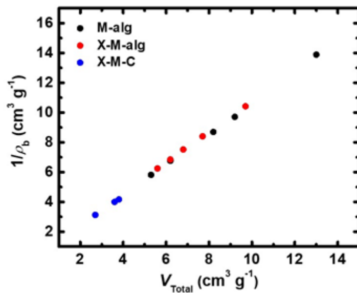
Figure S5. Plot of 1/\rho_b vs V_{Total} for native (M-alg), crosslinked (X-M-alg) and carbon (X-M-C) aerogels, as indicated.
