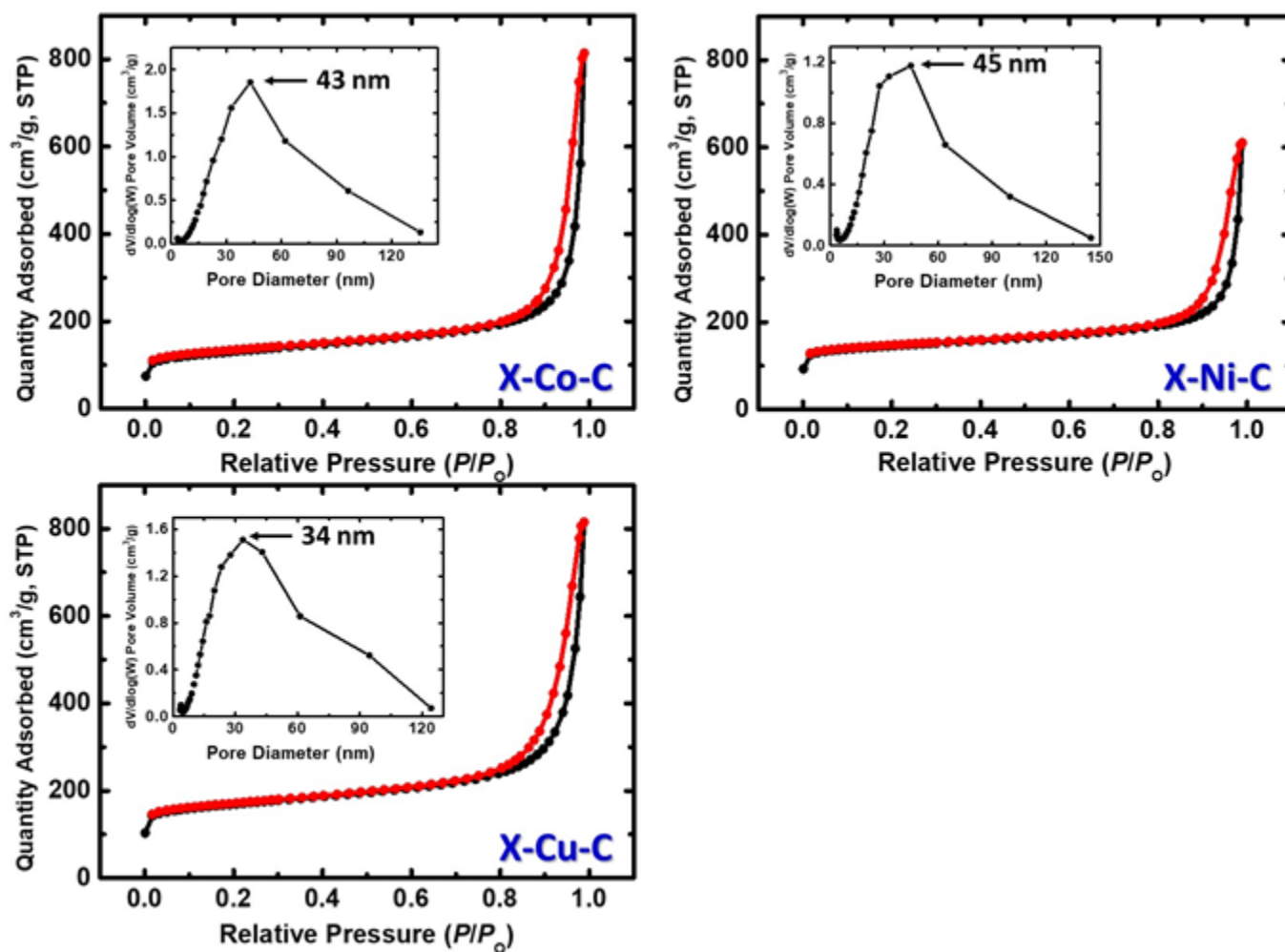
Figure S14. N 2 -sorption diagrams of carbon (X-M-C; M: Co, Ni, Cu) aerogel beads, as indicated. Insets show pore size distributions by the BJH method.
