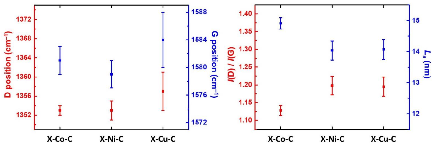
Figure S11. Left: Position of D and G bands on the Raman spectra of carbon (X-M-C; M: Co, Ni, Cu) aerogel beads. Right: I(D)/I(G) peak intensity ratio and calculated crystallite size ( L_a ) of the graphitic domains. Error bars stand for standard deviation (N=10).
