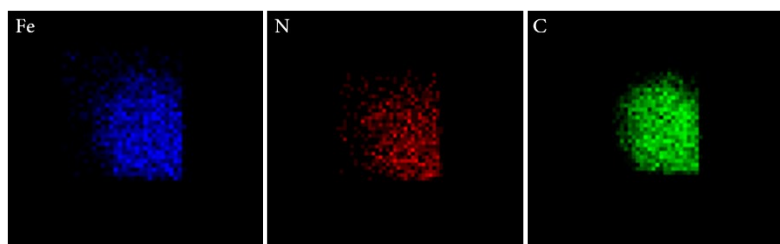
Figure S1 Element mapping for the NGC-Fe sample.
