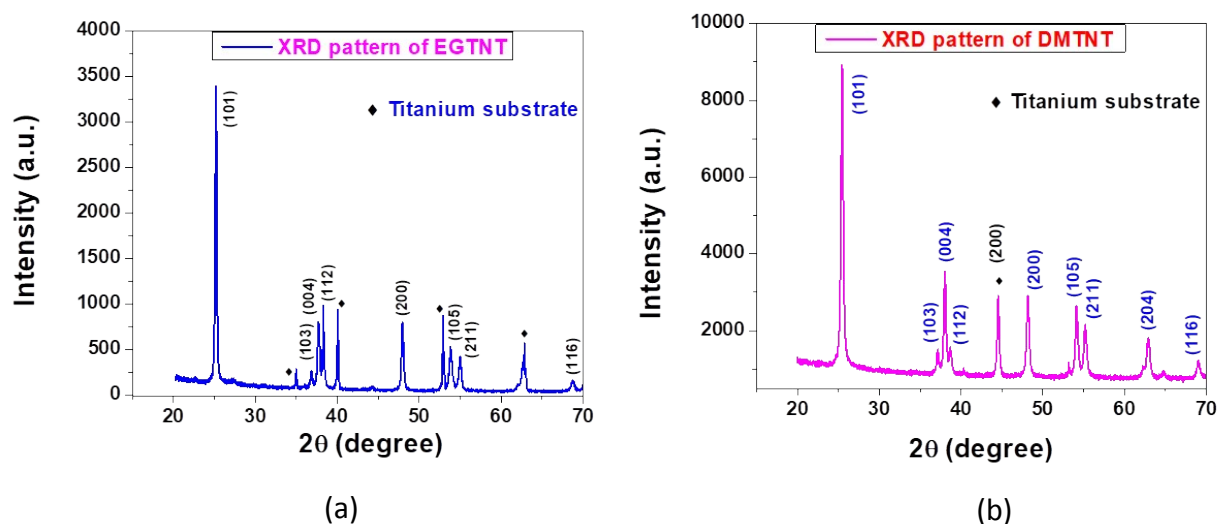
Fig. S1. XRD patterns of (a) EGTNT and (b) DMTNT confirming the anatase phase of both types of nanotube. The peaks are matched with JCPDS card no. 01-071-1169 and 01-073-1764 respectively for matching with anatase phase.
