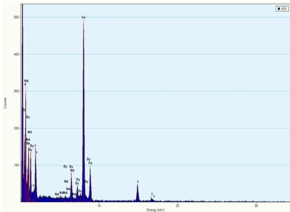
Fig. S1 The energy dispersive X-ray spectroscopy of NaYF 4 : Nd/NaDyF 4 NCs.
