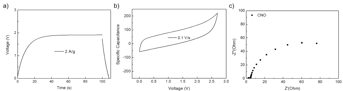
Figure S1. (a) Galvanostatic charge-discharge curves of CNO electrode with 1 M TEABF 4 electrolyte. (b) Cyclic voltammetry profile, (c) Nyquist plot
