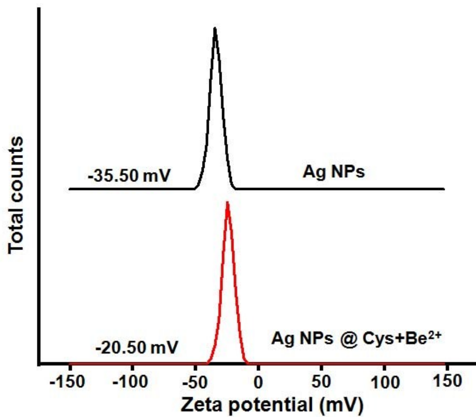
Fig S1. Zeta potential of the probe with and without analyte
