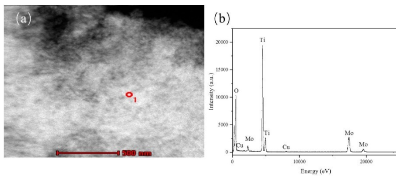
Fig. S1 EDX spectra of Cu/TiO 2 -1.0%
