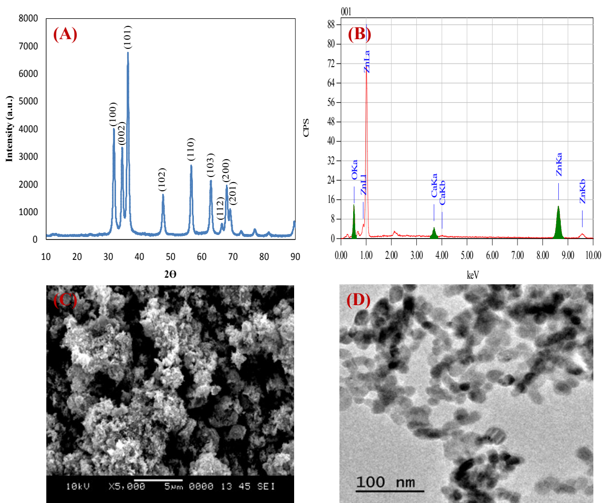
Fig. S1. (A) X-ray Diffraction patterns, (B) Energy-dispersive X-ray spectroscopy, (C) Scanning electron microscopy, (D) Transmission electron microscopy images of 5% Ca-doped ZnO nanoparticles.
