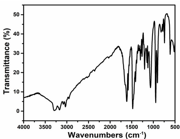
Figure S1. The IR spectrum of 1
