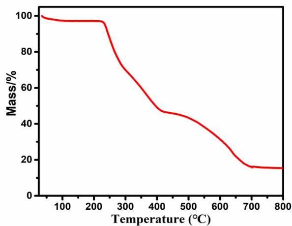
Figure S2. The TG cure of compound 1 .
