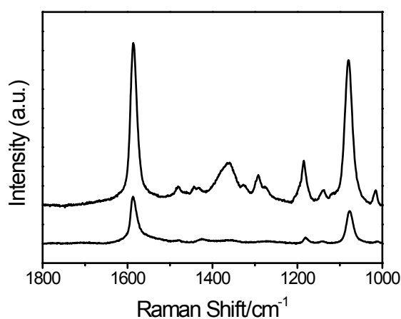
Figure S1. SERS spectra of 4-MBA ( 10^{-3} mol/L) adsorbed on the PS/Au (10 min)/ZIF-8 and PS/Au (10 min) substrates under 633 nm laser line.
