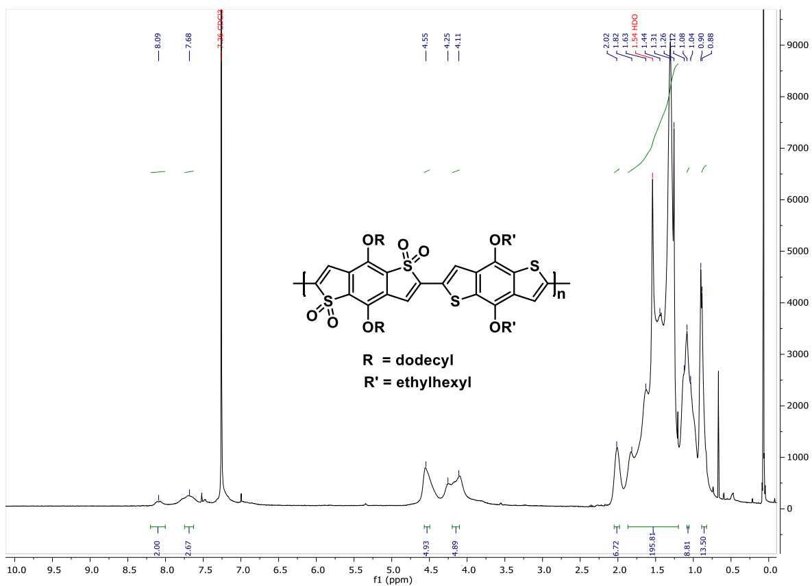
Figure S4: 1 H NMR of PBDTT-BDT
