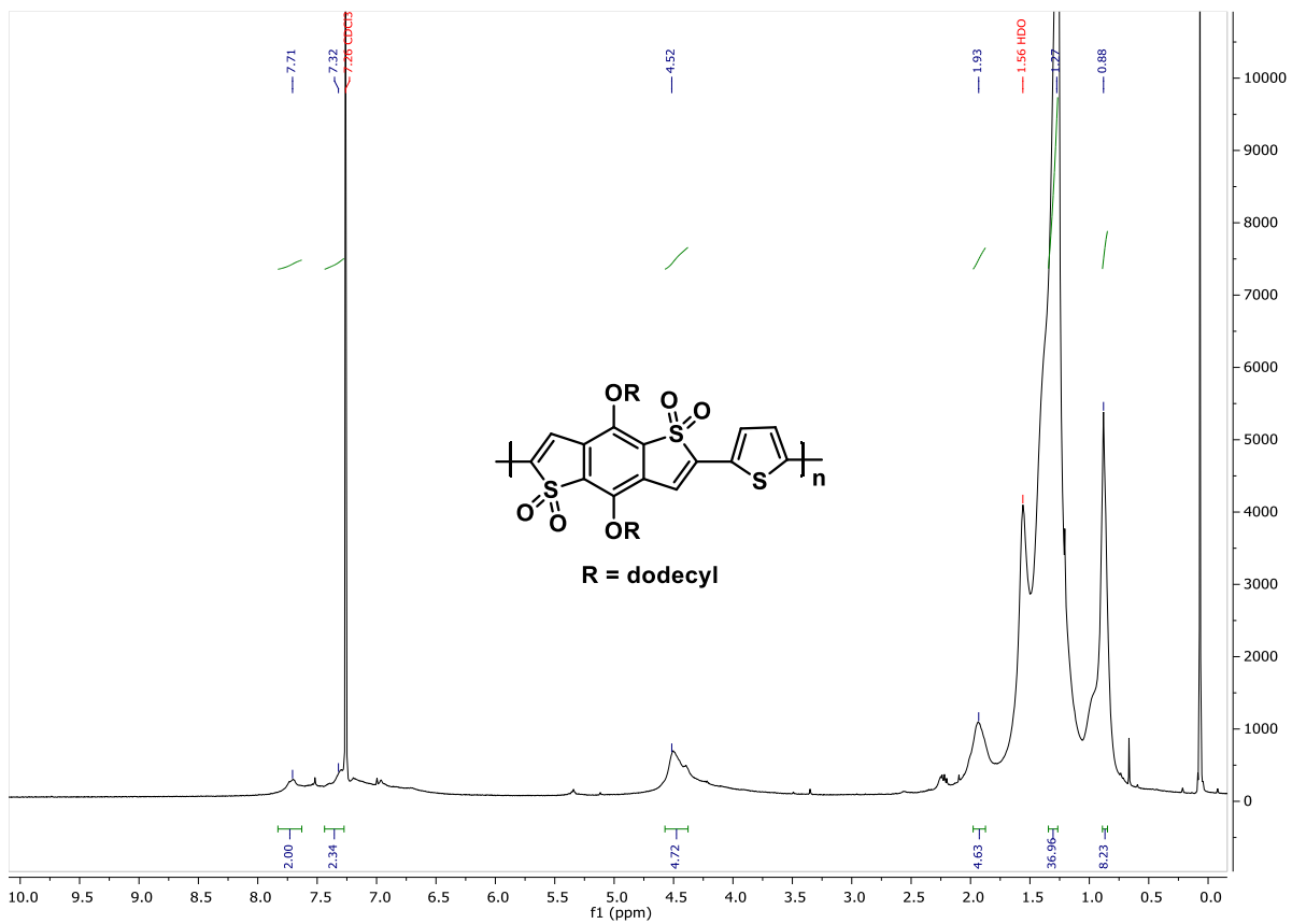
Figure S3: 1 H NMR of PBDTT-Th
