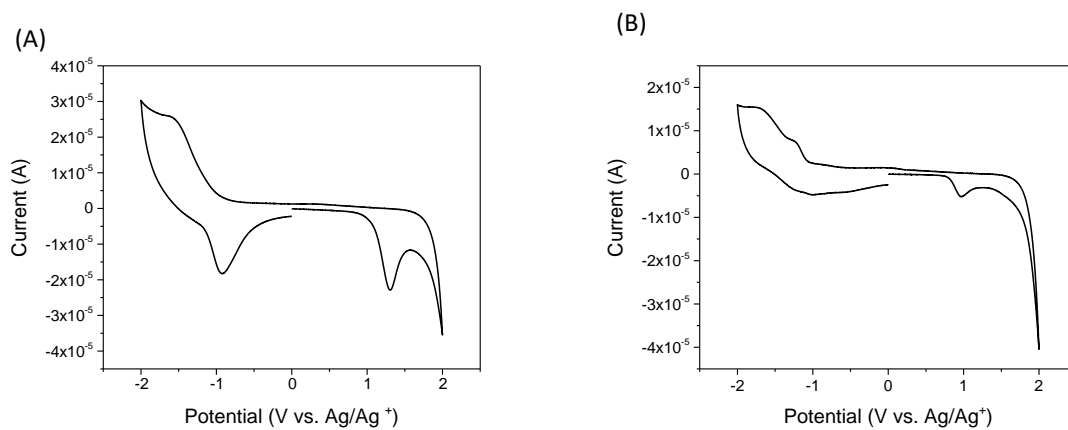
Figure S5: CV spectra of (A) PBDTT-Th and (B) PBDTT-B
