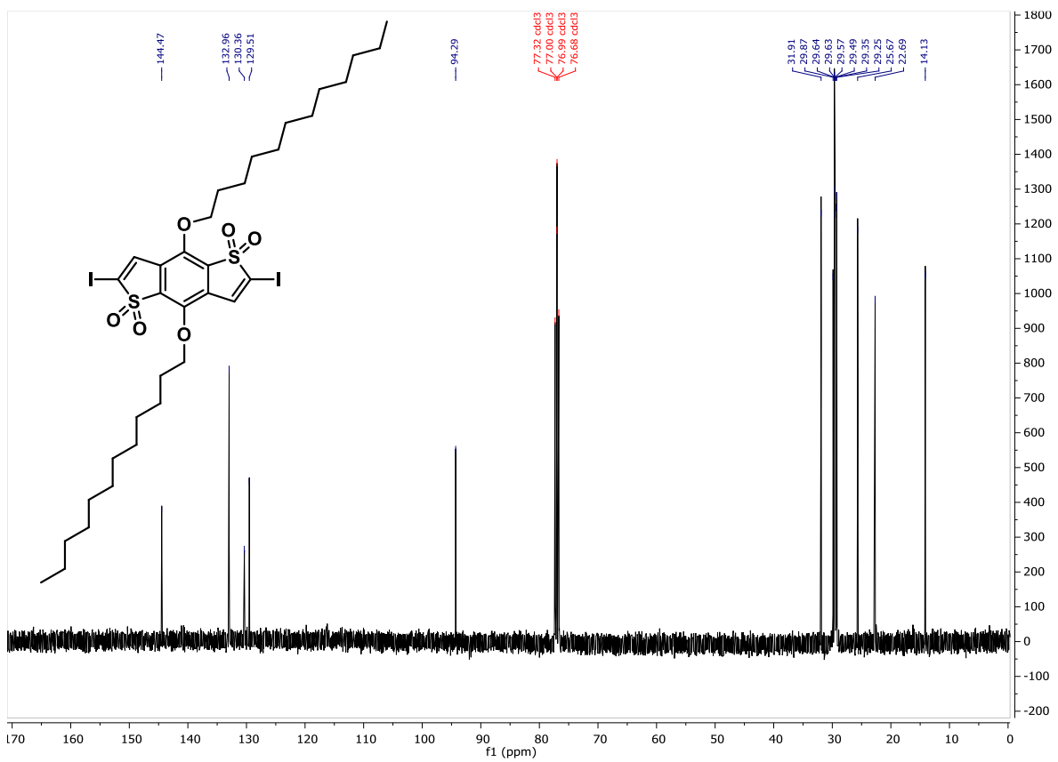
Figure S2: 13 C NMR of 2
