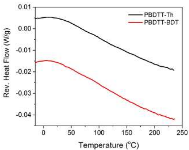
Figure S6: DSC thermograms of PBDTT-Th and PBDTT-BDT.
