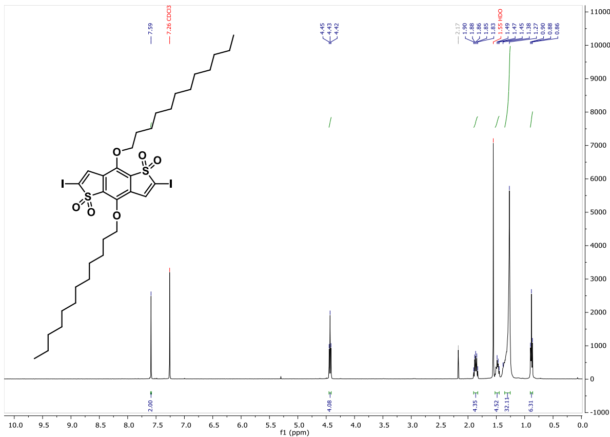
Figure S1: 1 H NMR of 2
