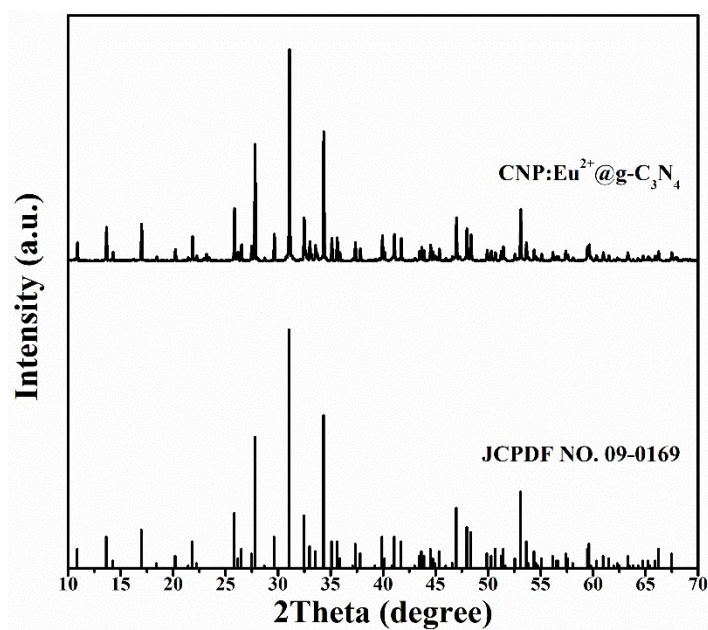
Figure S1 XRD pattern of the CNP:Eu 2+ @g-C 3 N 4 and standard card of \beta -Ca 3 PO 4 (JCPDS NO.09-0169).
