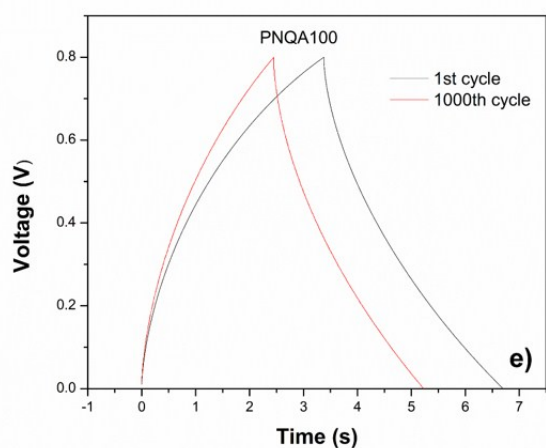
Fig S1. Stability of the supercapacitors by measuring galvanostatic charge discharge curves of the 1st and 1000th cycles for the a) PNQA10, b) Li-PNQA10, c) PNQA20, d) Li-PNQA20, e) PNQA100, f) Li-PNQA100 polyelectrolytes.
