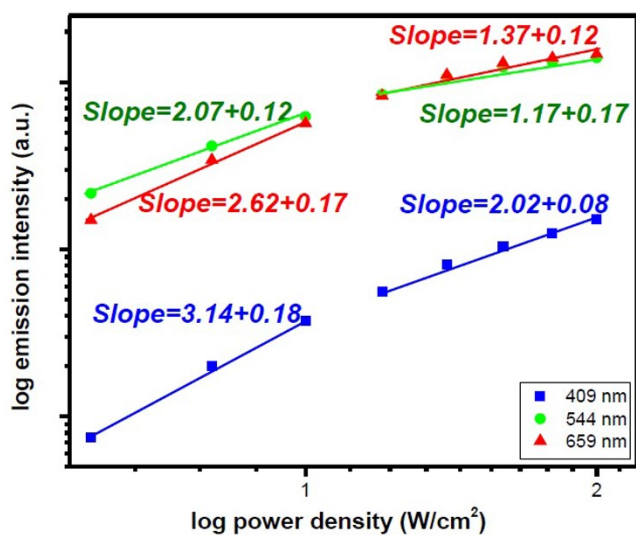
Figure S1) log-log plot of emission intensity of NaYF 4 :Yb,Er@ NaYF 4 versus excitation power density.
