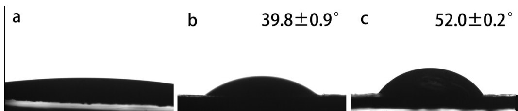
Fig. S3 The static contact angle of water droplet on the disks of LS/CTAB complexes with different molecular weight LS (a: LS/CTAB-a, b: LS/CTAB-b, c: LS/CTAB-c)
