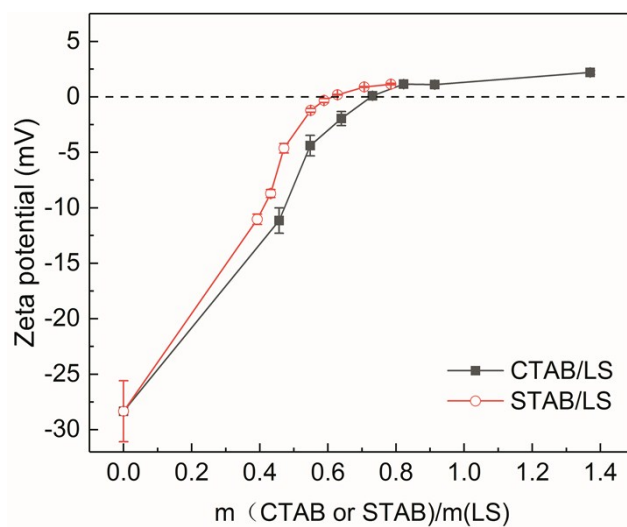
Fig. S1 Zeta potential of CTAB/LS and STAB/LS
