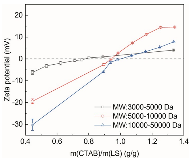
Fig. S2 Zeta potential of CTAB/LS with different molecular weight of LS
