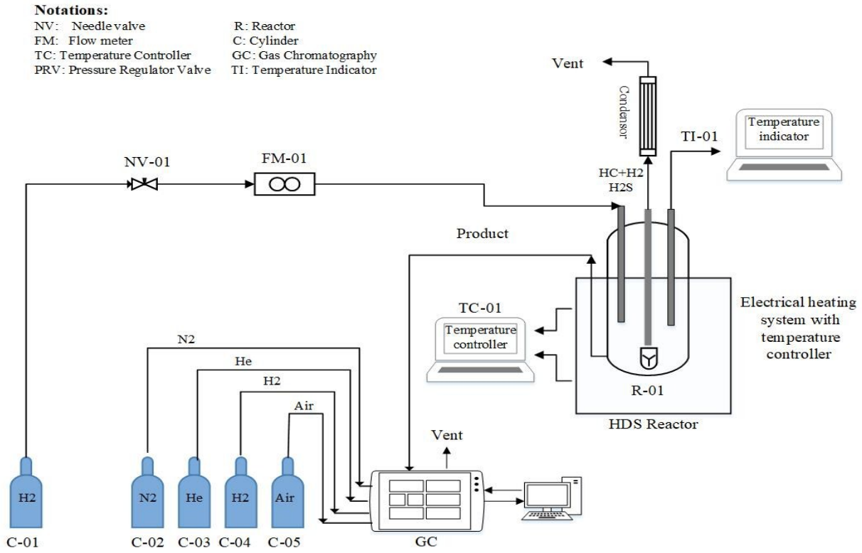
Figure 2.S. Schematic diagram of experimental setup toward hydrodesulfurization process over combusted NMACA-x nanocatalysts
