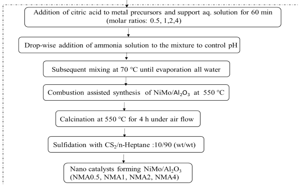
Figure 1.S. Preparation steps of combustion assisted synthesis of NiMo/Al 2 O 3
