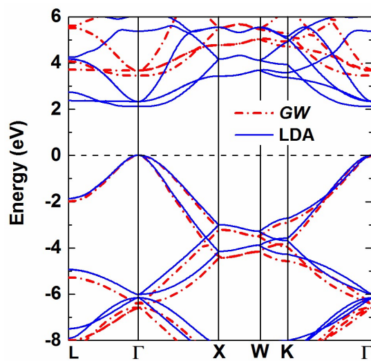
Fig. S1: The G_0W_0 and LDA band structures of T-carbon.
