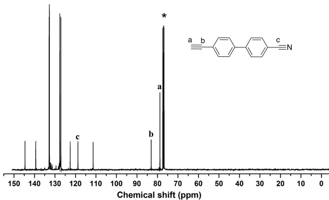
Figure S2 The ^{13}\text{C} -NMR spectrum of 4-Cyano-4'-ethynylbiphenyl in \text{CDCl}_3 .
