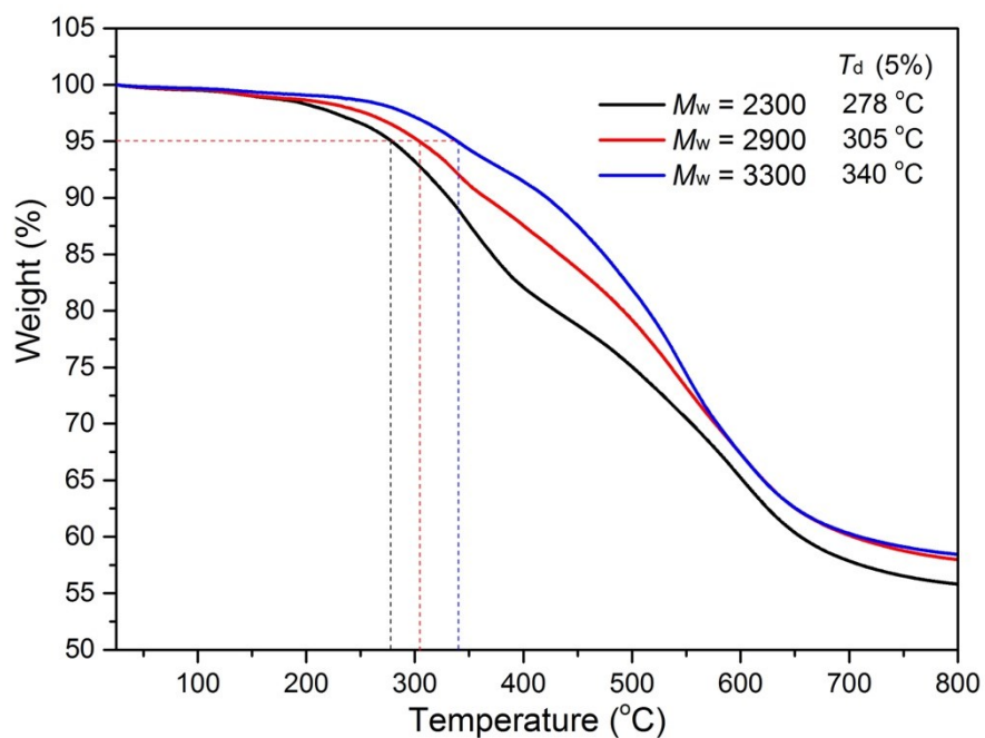
Figure S5 Thermograms of the polyoxazoles with different number average molecular weight ( M_w ). The measurements were performed under N_2 atmosphere at the heating rate of 10\text{ °C/min} .
