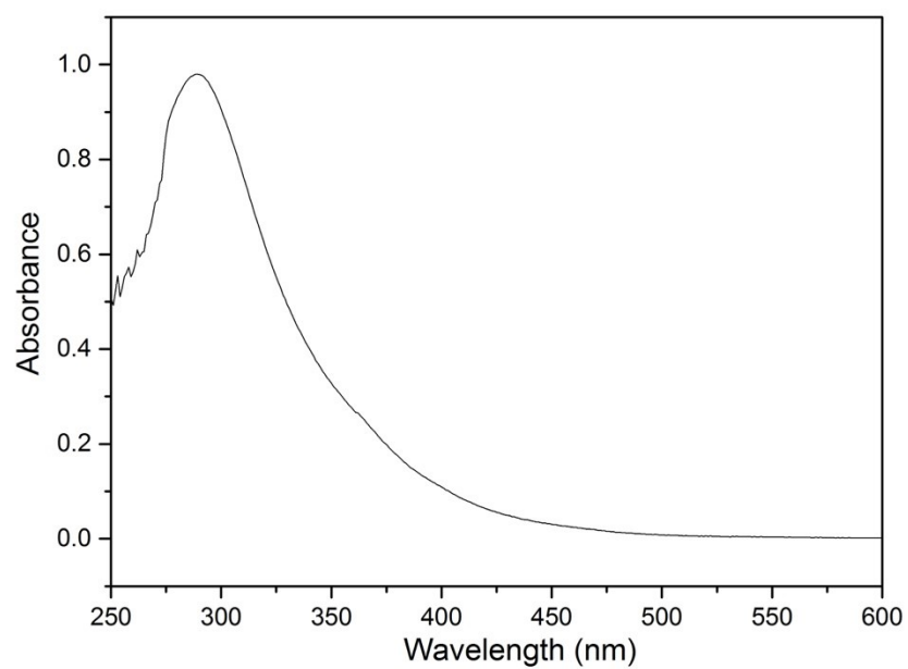
Figure S3 UV-vis absorbance spectra of the polyoxazoles in THF. Solution concentration: 1 \times 10^{-4} mol / L.
