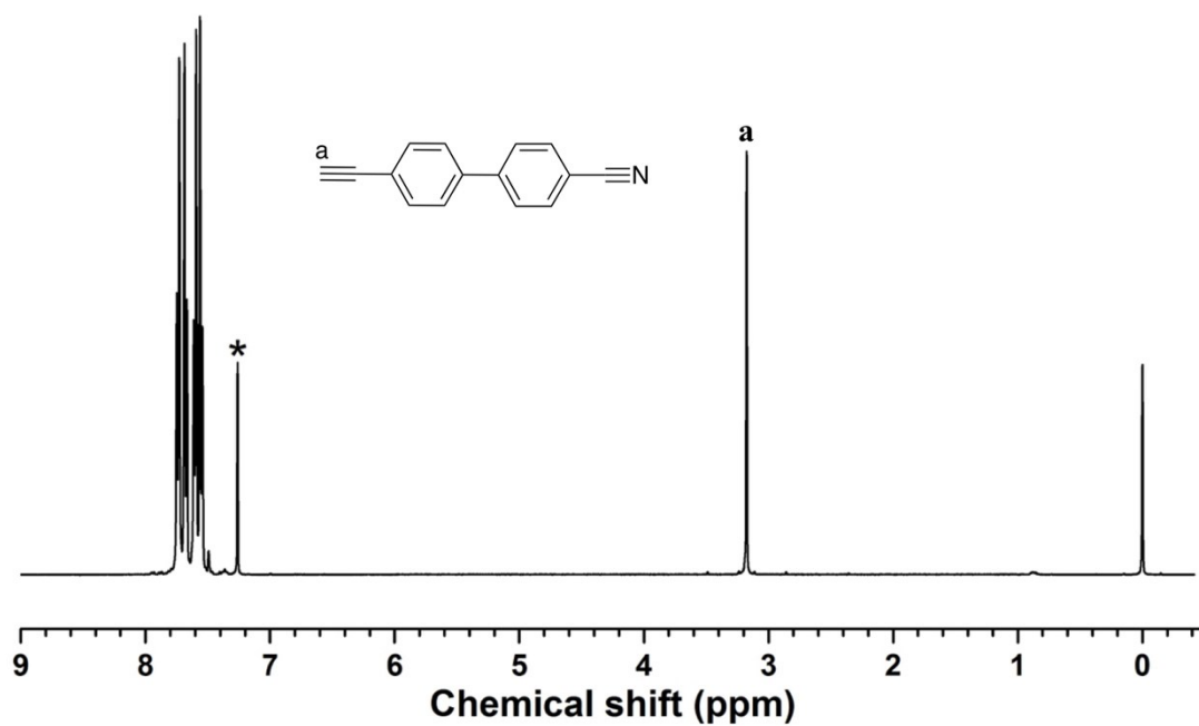
Figure S1 The ^1\text{H} -NMR spectrum of 4-Cyano-4'-ethynylbiphenyl in \text{CDCl}_3 .
