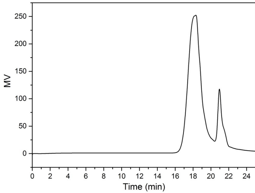
Figure SA12 The GPC result of entry 1 in Table 3.
