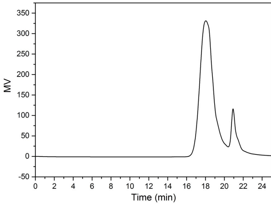
Figure SA14 The GPC result of entry 3 in Table 3.
