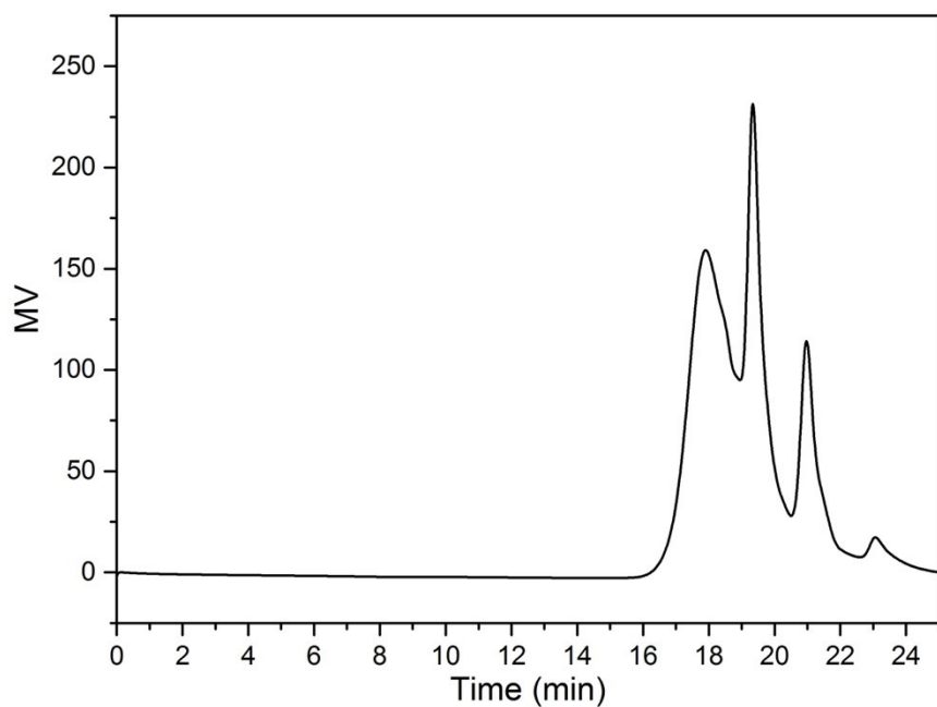
Figure SA1 The GPC result of entry 1 in Table 1.
