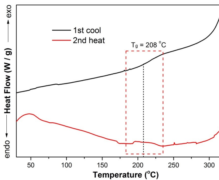
Figure S4 DSC of the polyoxazoles. The measurements were performed under N_2 atmosphere at the heating rate of 10 \text{ }^\circ\text{C}/\text{min} .
