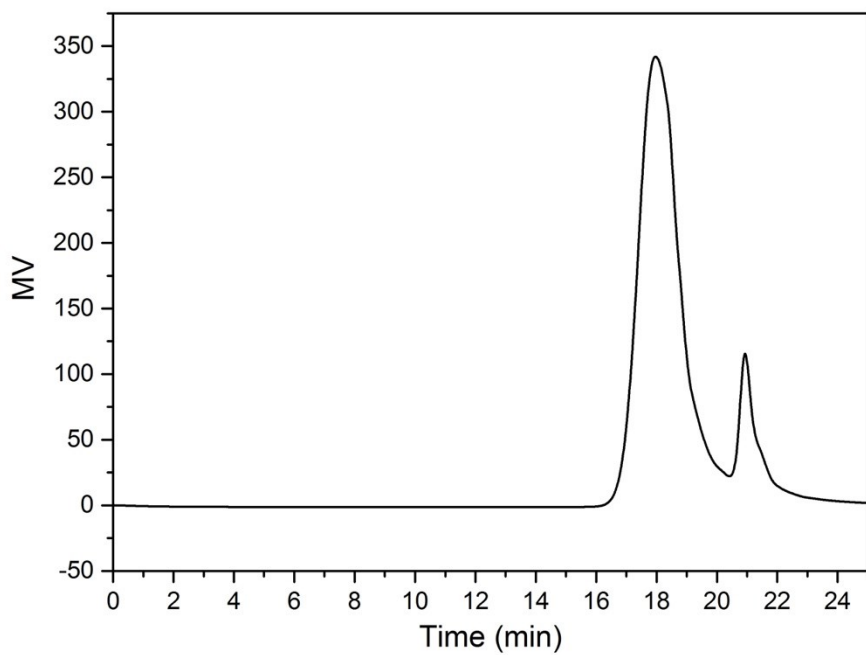
Figure SA21 The GPC result of entry 3 in Table 4.
