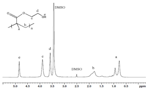
Fig. S1. 1 H NMR spectrum of PHEMA in DMSO-d 6 .
