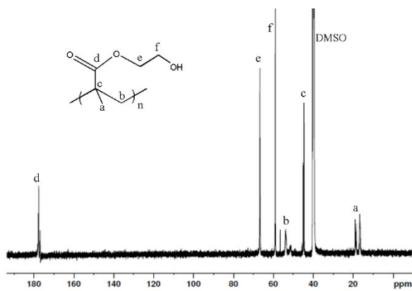
Fig. S2. 13 C NMR spectrum of PHEMA in DMSO-d 6 .
