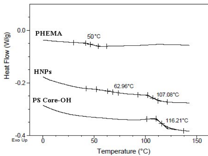
Fig. S4. DSC thermograms of HNP (PS Core-PHEMA), PS Core-OH, and PHEMA.
