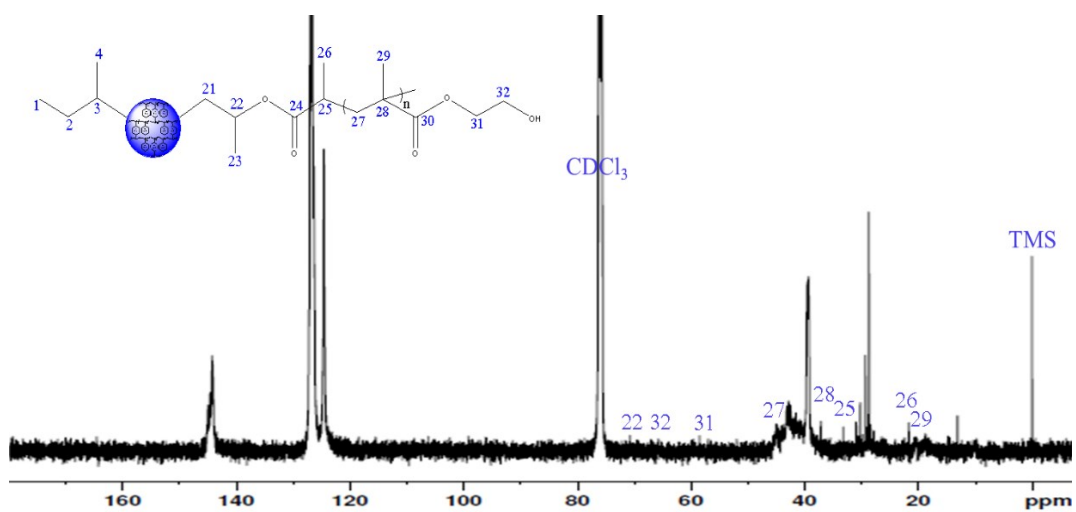
Fig. S3 ^{13}\text{C} NMR spectrum of PS Core-PHEMA in \text{CDCl}_3 .
