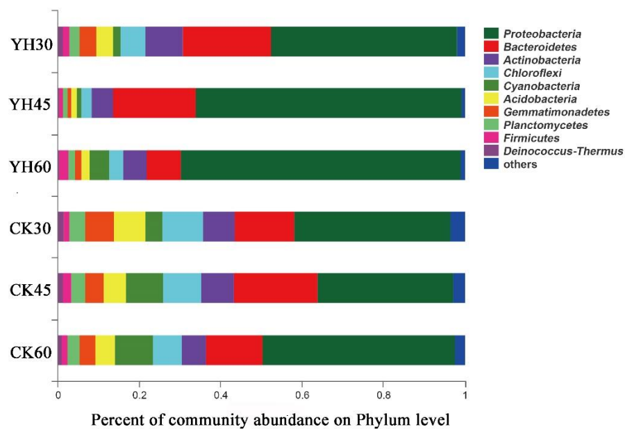
Fig. S1 Bacterial relative abundance of the species at the level of phylum
