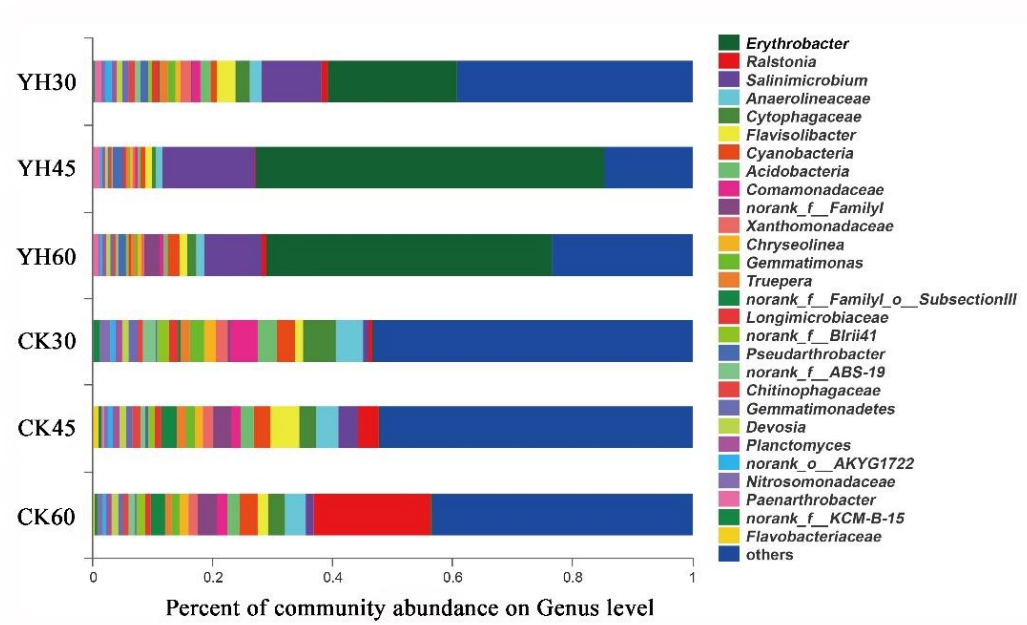
Fig. S2 Bacterial relative abundance of the species at the level of genus
