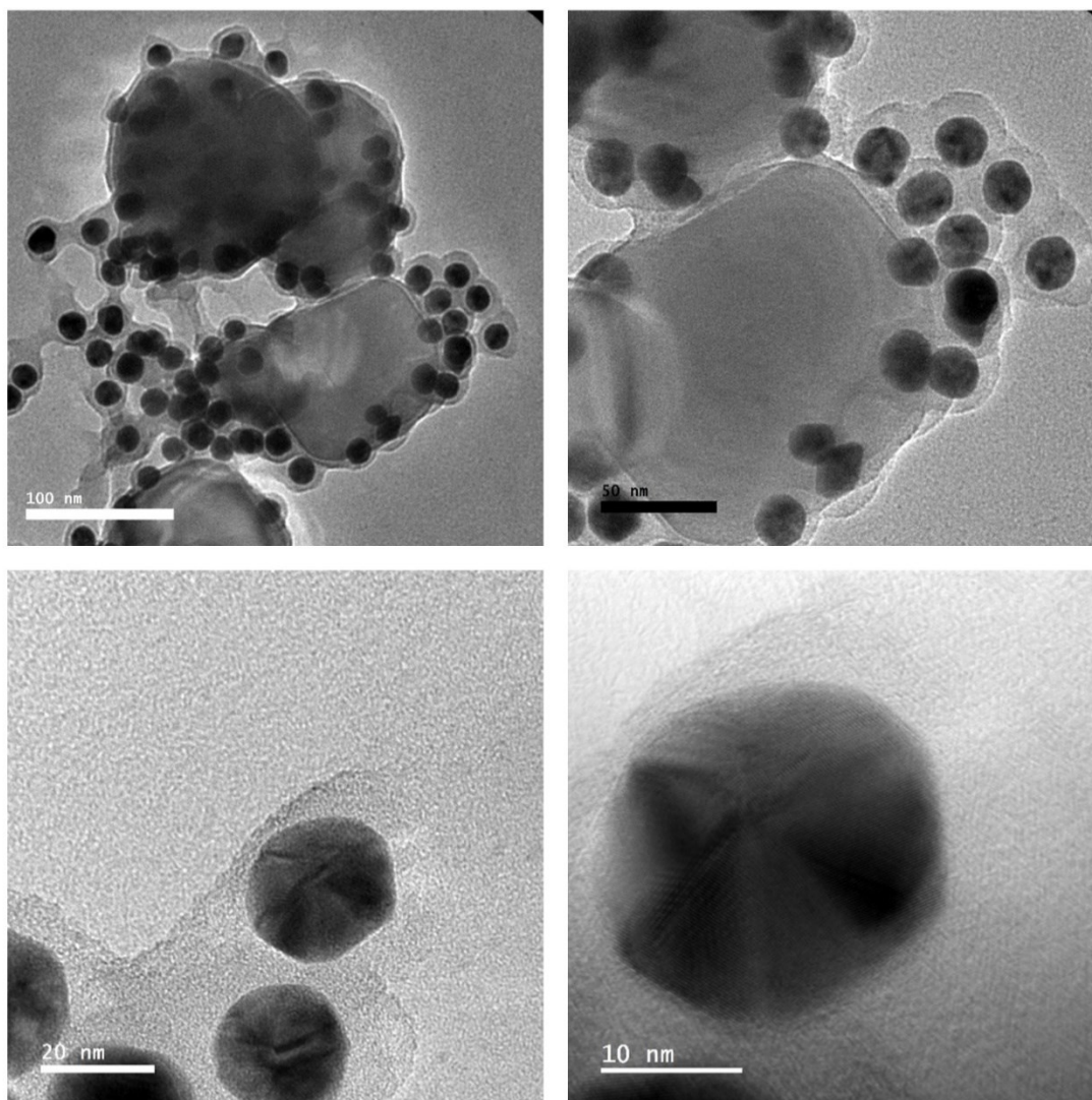
Figure S1. TEM images of Au/TiO 2 at varying levels of magnification
