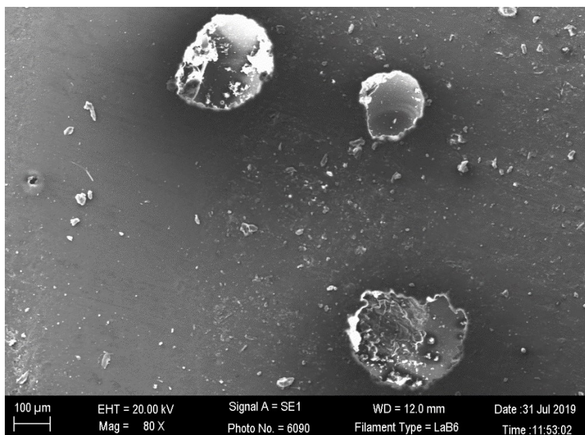
Figure S2. SEM image of broken DCPD-CNT-UF microcapsules on the surface of epoxy resin cast specimen
