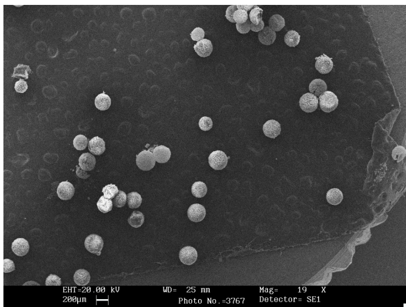
Figure S1. SEM image showing the cluster of DCPD-CNT-UF microcapsules
