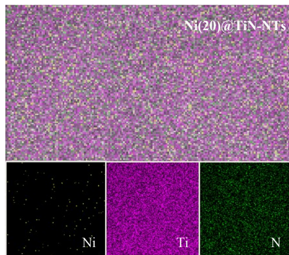
Fig.S1 SEM - mapping image of as-fabricated catalyst Ni(20)@TiN-NTs
