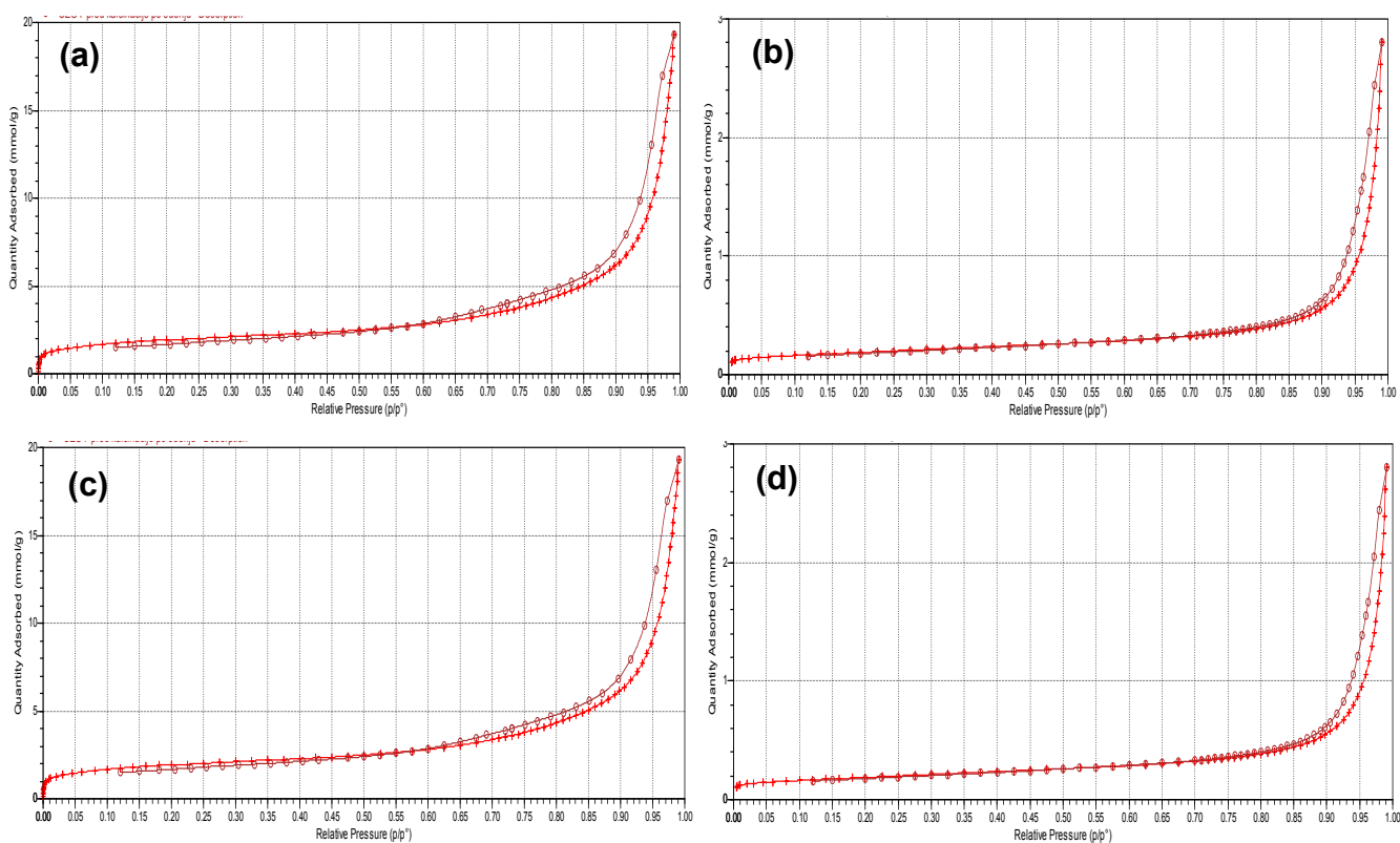
Figure S1: N 2 physisorption isotherms of (a) Cu-Fe/Al 2 O 3 , (b) CuFe 2 O 4 , (c) Cu/CuFe 2 O 4 and (d) Fe/CuFe 2 O 4 catalyst
