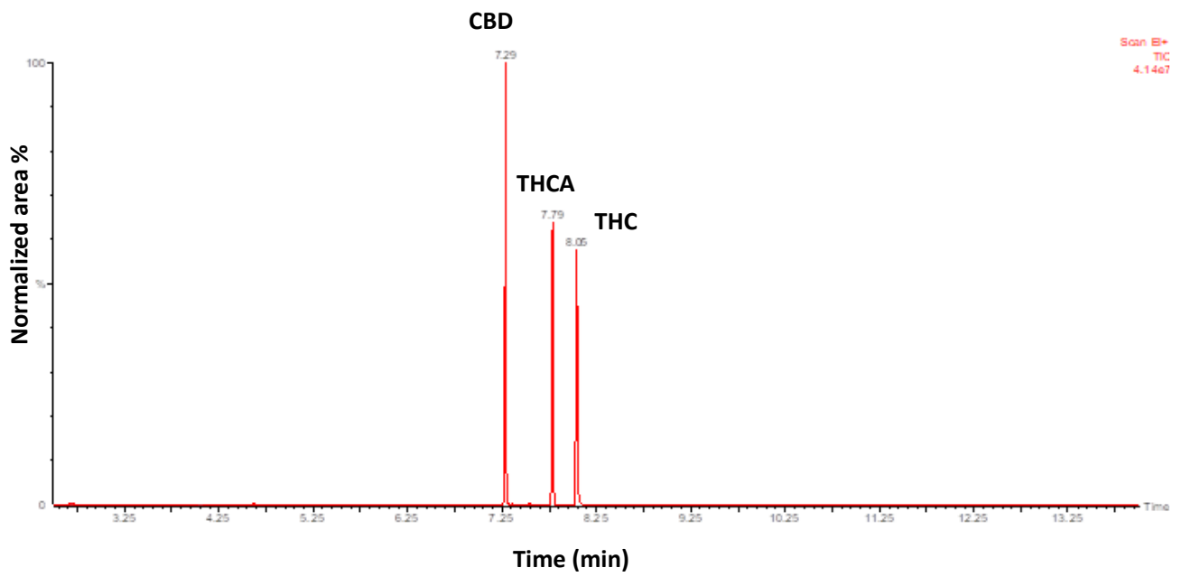
Figure 3S. Total Ion Chromatogram (TIC) of the standard mix of cannabinoids
