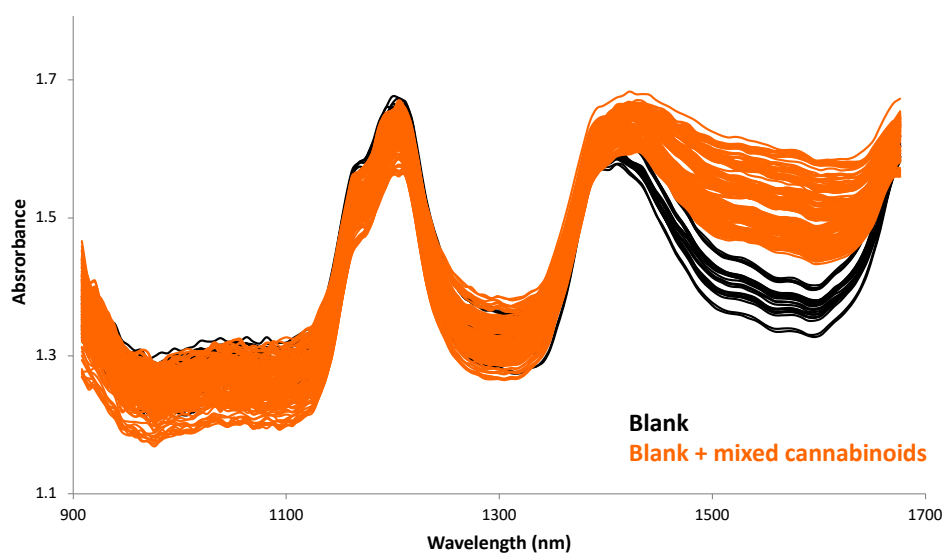
Figure 2S. Collected spectra of oils (black) and oils fortified with a mixed solution of THC, THCA and CBD (orange)
