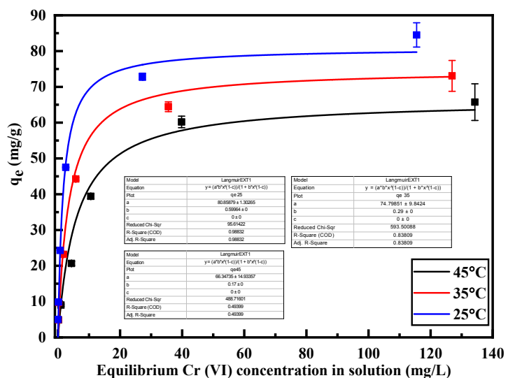
Fig1. Showing Non-Linear Langmuir Fit.
