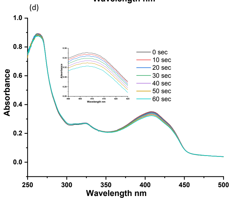
Figure S2 UV-visible spectra of DPBF (a) blank (b) PTh/BQ-MS, (c) PTh/BQ-US, (d) PTh/BQ-MW
