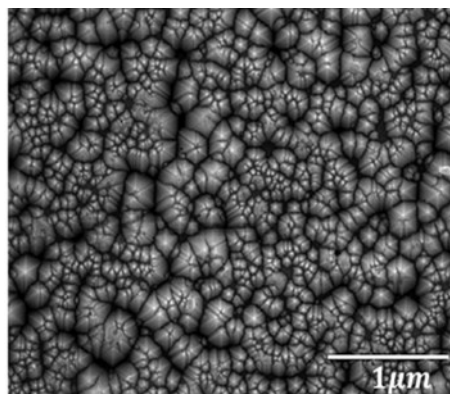
Fig. S2 Scanning electron microscopy top-view image of the KOH-etched surface of Sample A.
