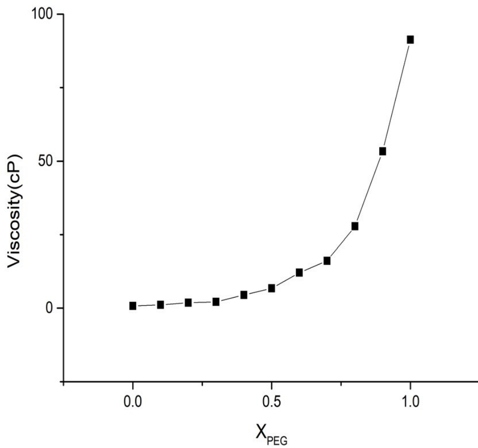
Figure S2. Graph of the viscosity in different PEG fraction.
