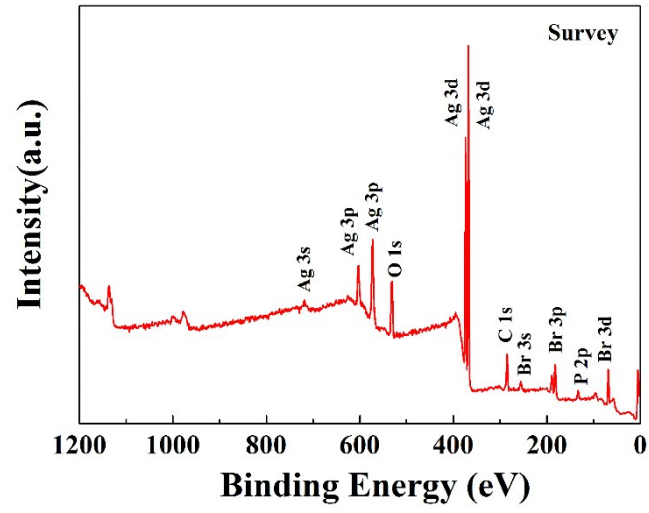
Figure S2 XPS survey spectrum of ABAP-48%
