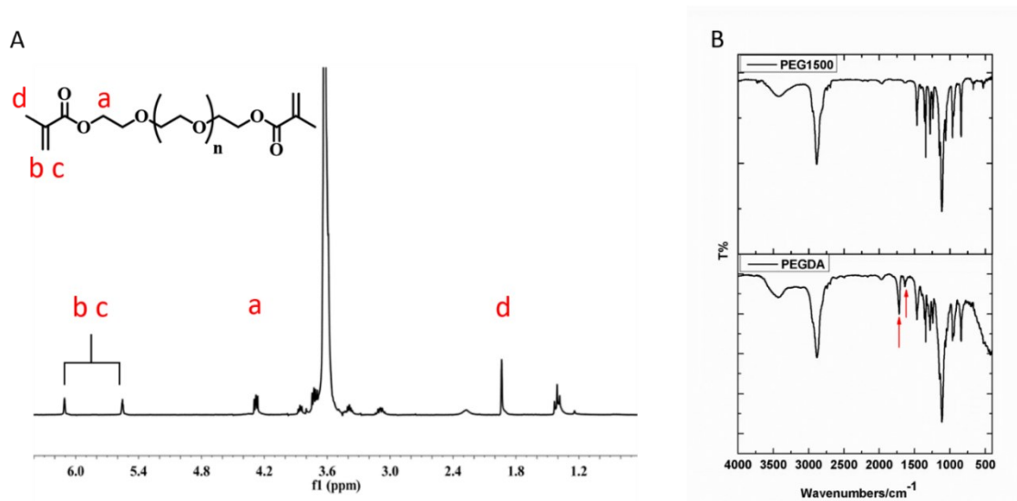
Figure S1. ^1\text{H-NMR} of PEGDA (A) and IR spectra of PEG1500 and PEGDA (B).
